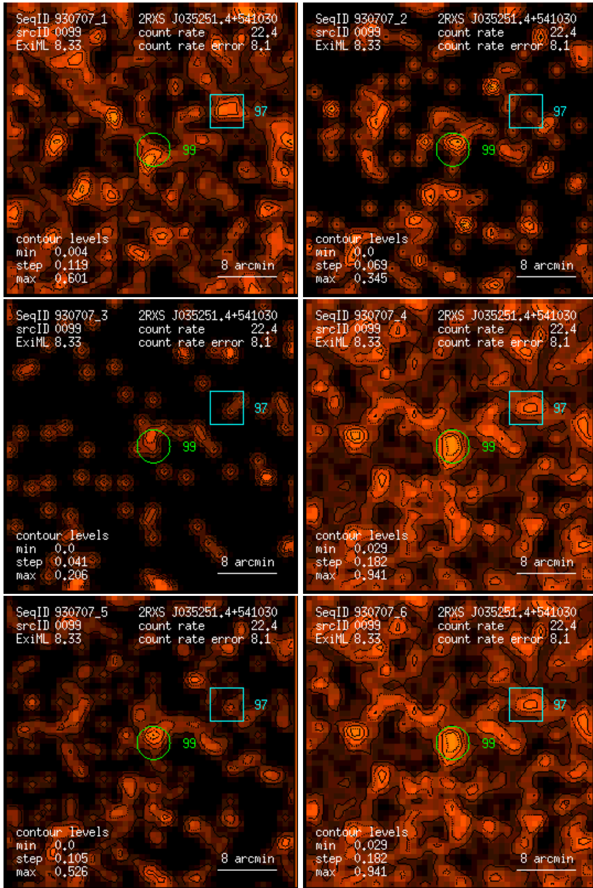
Figure 99: RASS 930707: detection 0099: band rate images, Gaussian filter: (1) PSPC channels 11 – 41, (2) 52 – 90, (3) 91 – 201, (4) 11 – 235, (5) 52 – 201, (6) 11 – 201. Broad band rates in counts/ks. Band rate contour levels in counts/ks/arcmin 2 .
