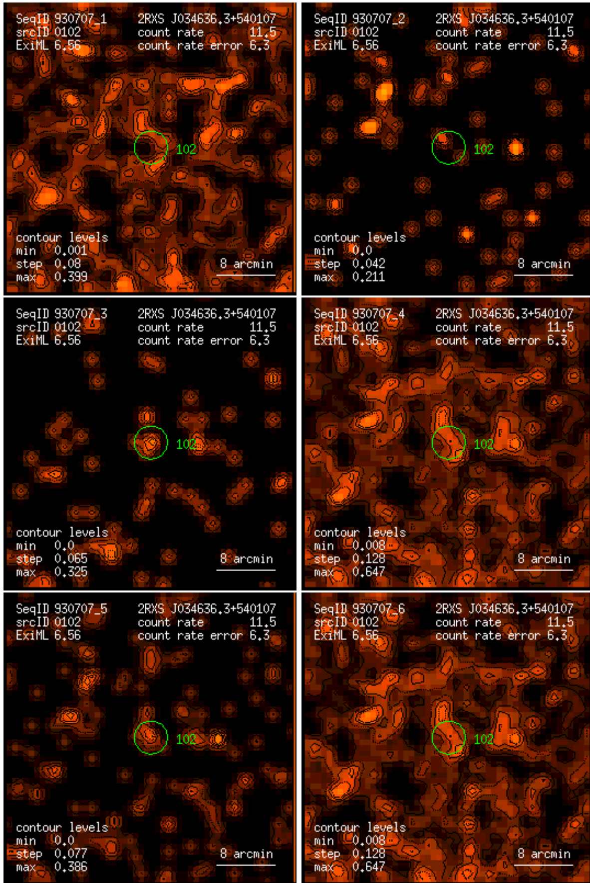
Figure 102: RASS 930707: detection 0102: band rate images, Gaussian filter: (1) PSPC channels 11 – 41, (2) 52 – 90, (3) 91 – 201, (4) 11 – 235, (5) 52 – 201, (6) 11 – 201. Broad band rates in counts/ks. Band rate contour levels in counts/ks/arcmin 2 .
