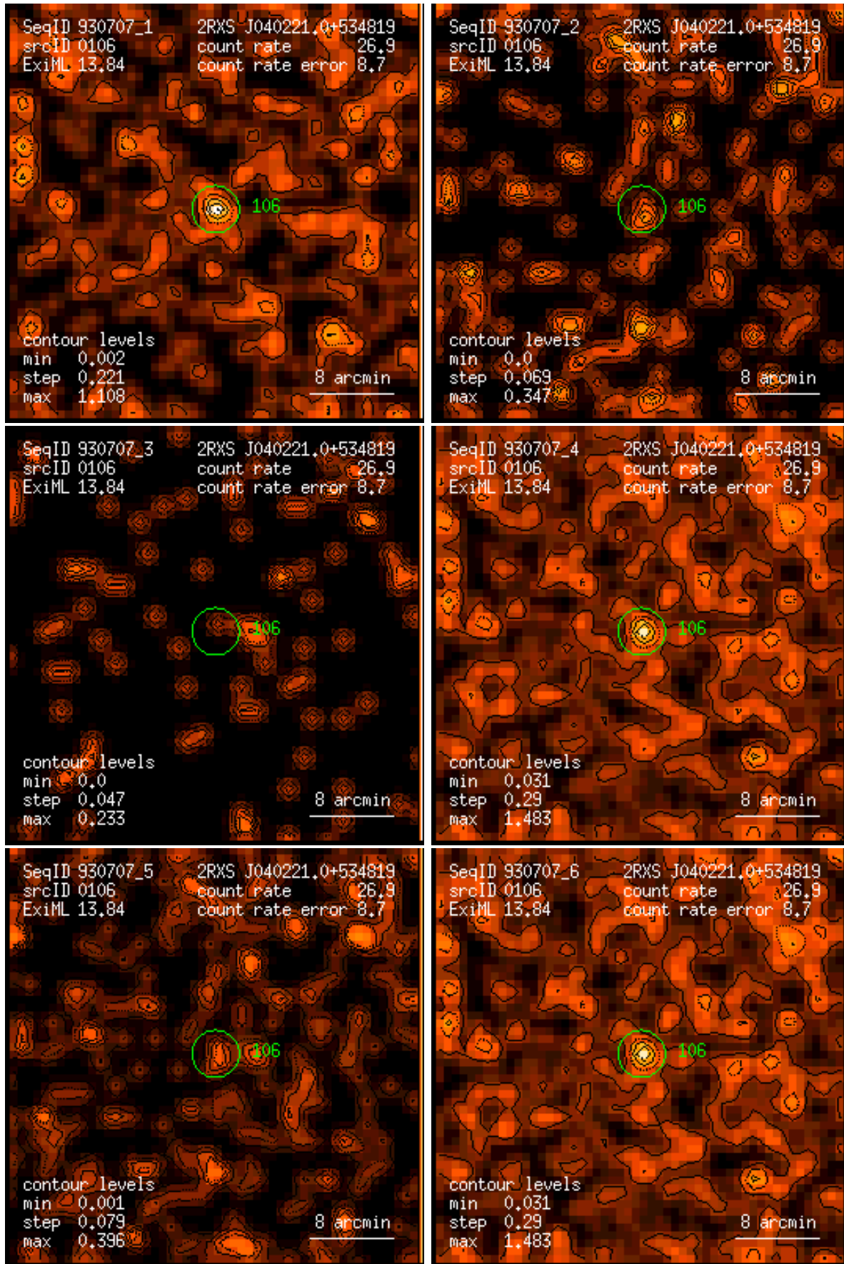
Figure 106: RASS 930707: detection 0106: band rate images, Gaussian filter: (1) PSPC channels 11 – 41, (2) 52 – 90, (3) 91 – 201, (4) 11 – 235, (5) 52 – 201, (6) 11 – 201. Broad band rates in counts/ks. Band rate contour levels in counts/ks/arcmin 2 .
