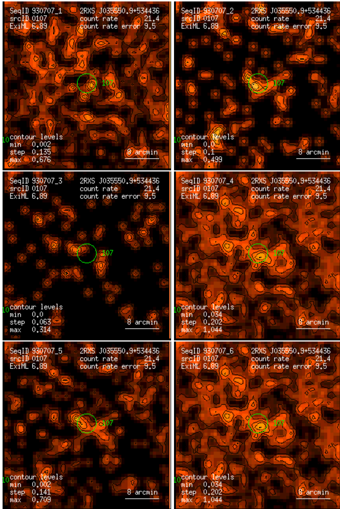
Figure 107: RASS 930707: detection 0107: band rate images, Gaussian filter: (1) PSPC channels 11 – 41, (2) 52 – 90, (3) 91 – 201, (4) 11 – 235, (5) 52 – 201, (6) 11 – 201. Broad band rates in counts/ks. Band rate contour levels in counts/ks/arcmin 2 .
