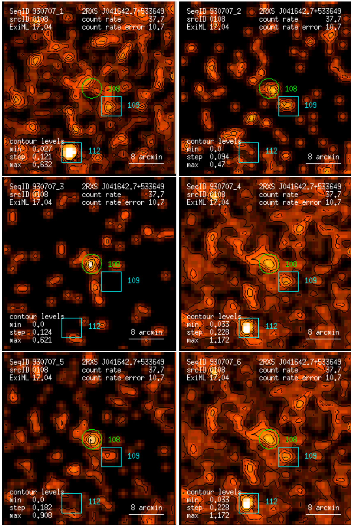
Figure 108: RASS 930707: detection 0108: band rate images, Gaussian filter: (1) PSPC channels 11 – 41, (2) 52 – 90, (3) 91 – 201, (4) 11 – 235, (5) 52 – 201, (6) 11 – 201. Broad band rates in counts/ks. Band rate contour levels in counts/ks/arcmin 2 .
