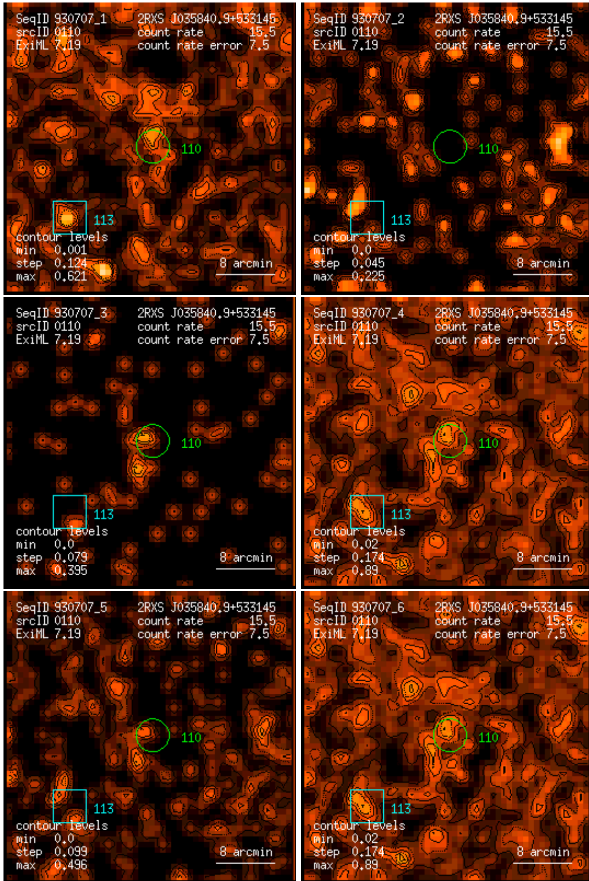
Figure 110: RASS 930707: detection 0110: band rate images, Gaussian filter: (1) PSPC channels 11 – 41, (2) 52 – 90, (3) 91 – 201, (4) 11 – 235, (5) 52 – 201, (6) 11 – 201. Broad band rates in counts/ks. Band rate contour levels in counts/ks/arcmin 2 .
