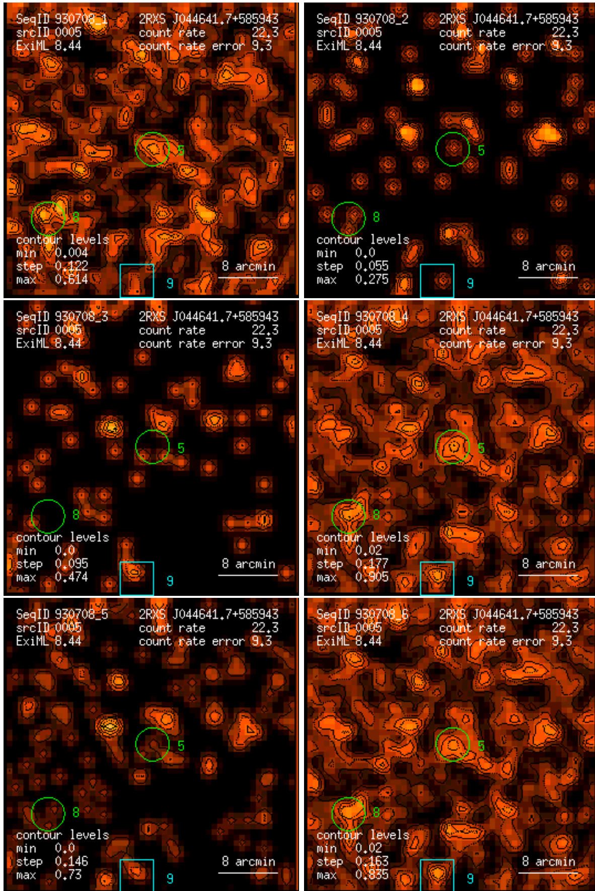
Figure 5: RASS 930708: detection 0005: band rate images, Gaussian filter: (1) PSPC channels 11 – 41, (2) 52 – 90, (3) 91 – 201, (4) 11 – 235, (5) 52 – 201, (6) 11 – 201. Broad band rates in counts/ks. Band rate contour levels in counts/ks/arcmin 2 .
