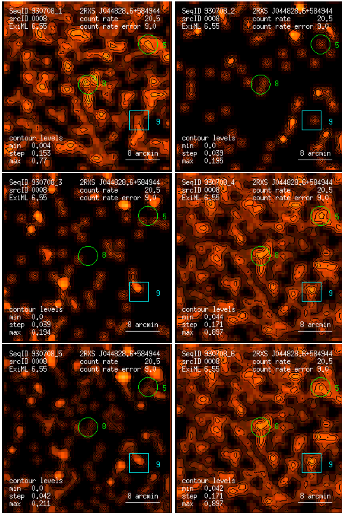
Figure 8: RASS 930708: detection 0008: band rate images, Gaussian filter: (1) PSPC channels 11 – 41, (2) 52 – 90, (3) 91 – 201, (4) 11 – 235, (5) 52 – 201, (6) 11 – 201. Broad band rates in counts/ks. Band rate contour levels in counts/ks/arcmin 2 .
