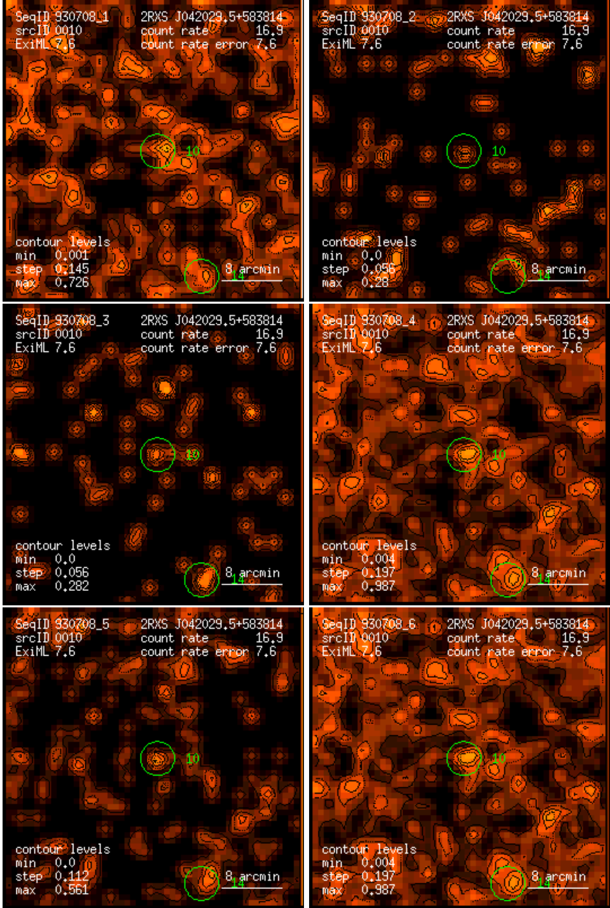
Figure 10: RASS 930708: detection 0010: band rate images, Gaussian filter: (1) PSPC channels 11 – 41, (2) 52 – 90, (3) 91 – 201, (4) 11 – 235, (5) 52 – 201, (6) 11 – 201. Broad band rates in counts/ks. Band rate contour levels in counts/ks/arcmin 2 .
