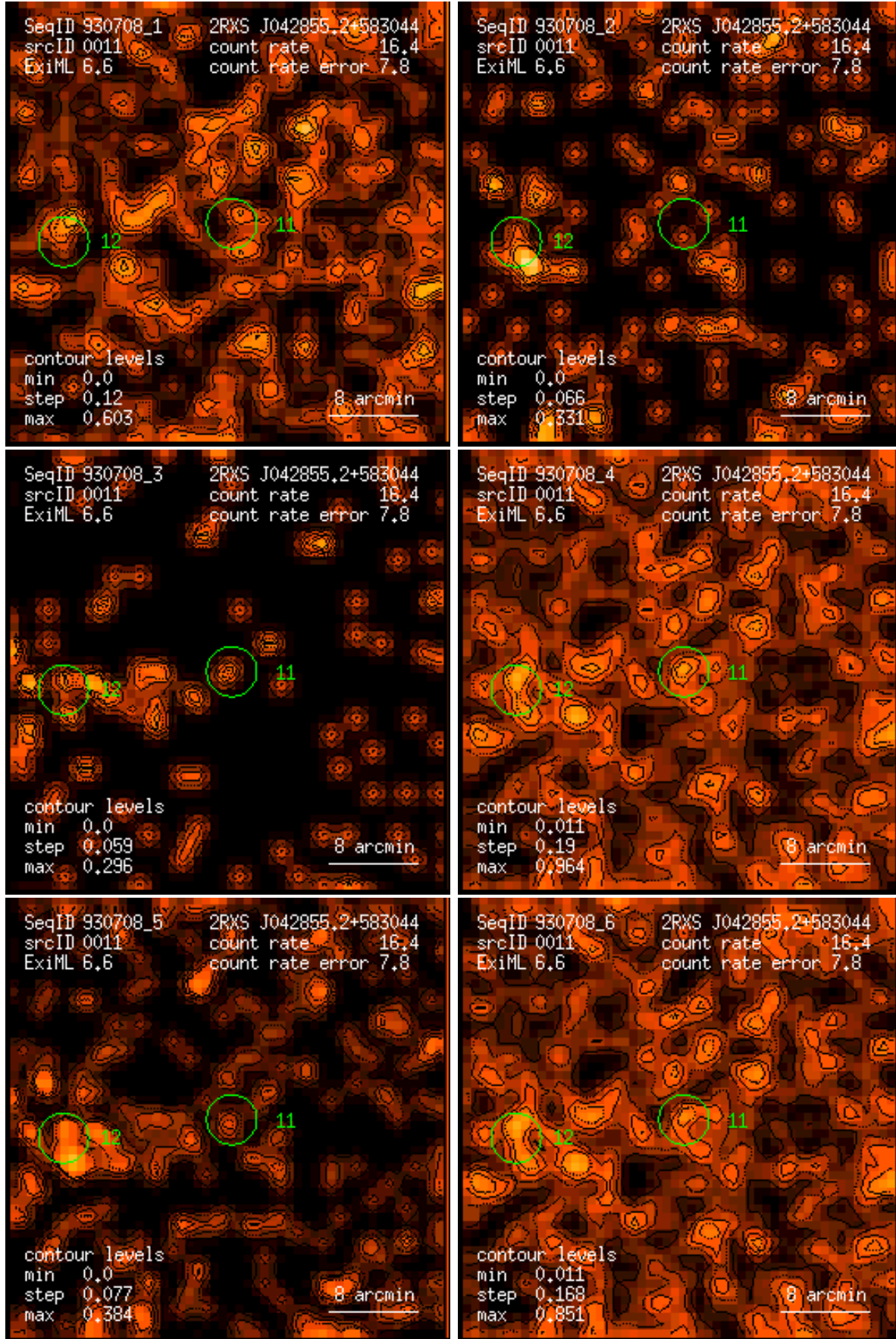
Figure 11: RASS 930708: detection 0011: band rate images, Gaussian filter: (1) PSPC channels 11 – 41, (2) 52 – 90, (3) 91 – 201, (4) 11 – 235, (5) 52 – 201, (6) 11 – 201. Broad band rates in counts/ks. Band rate contour levels in counts/ks/arcmin 2 .
