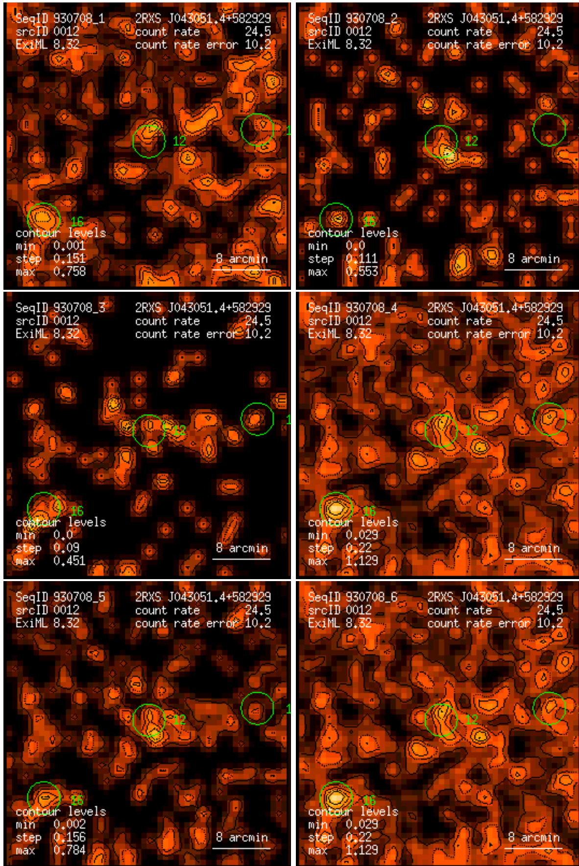
Figure 12: RASS 930708: detection 0012: band rate images, Gaussian filter: (1) PSPC channels 11 – 41, (2) 52 – 90, (3) 91 – 201, (4) 11 – 235, (5) 52 – 201, (6) 11 – 201. Broad band rates in counts/ks. Band rate contour levels in counts/ks/arcmin 2 .
