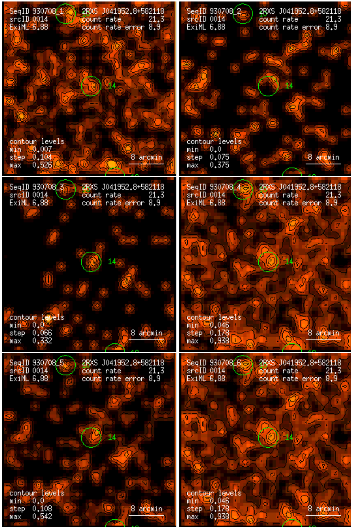
Figure 14: RASS 930708: detection 0014: band rate images, Gaussian filter: (1) PSPC channels 11 – 41, (2) 52 – 90, (3) 91 – 201, (4) 11 – 235, (5) 52 – 201, (6) 11 – 201. Broad band rates in counts/ks. Band rate contour levels in counts/ks/arcmin 2 .
