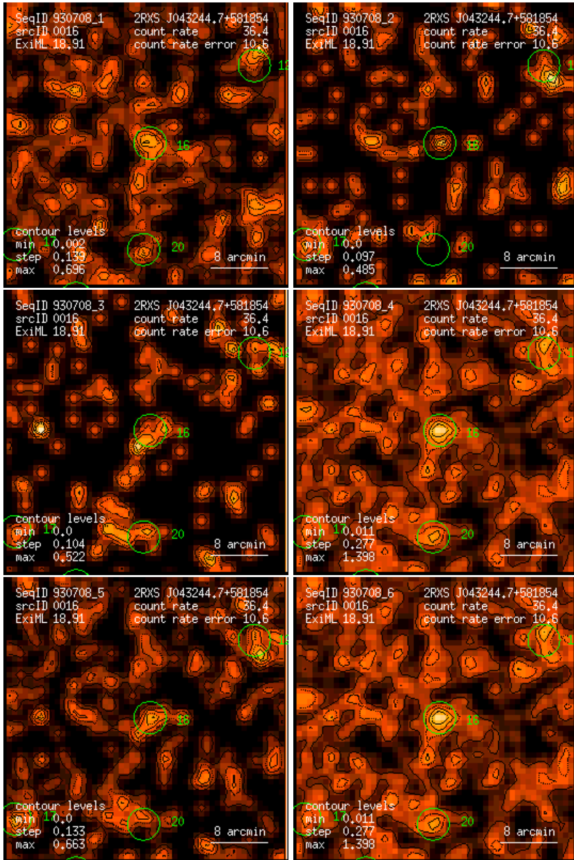
Figure 16: RASS 930708: detection 0016: band rate images, Gaussian filter: (1) PSPC channels 11 – 41, (2) 52 – 90, (3) 91 – 201, (4) 11 – 235, (5) 52 – 201, (6) 11 – 201. Broad band rates in counts/ks. Band rate contour levels in counts/ks/arcmin 2 .
