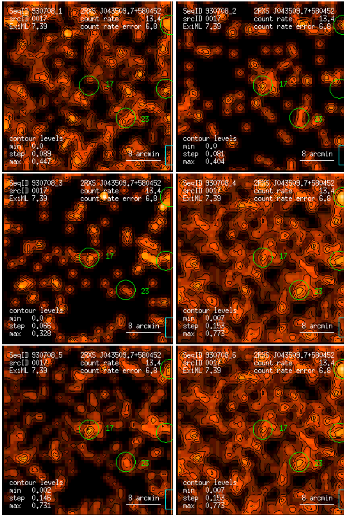
Figure 17: RASS 930708: detection 0017: band rate images, Gaussian filter: (1) PSPC channels 11 – 41, (2) 52 – 90, (3) 91 – 201, (4) 11 – 235, (5) 52 – 201, (6) 11 – 201. Broad band rates in counts/ks. Band rate contour levels in counts/ks/arcmin 2 .
