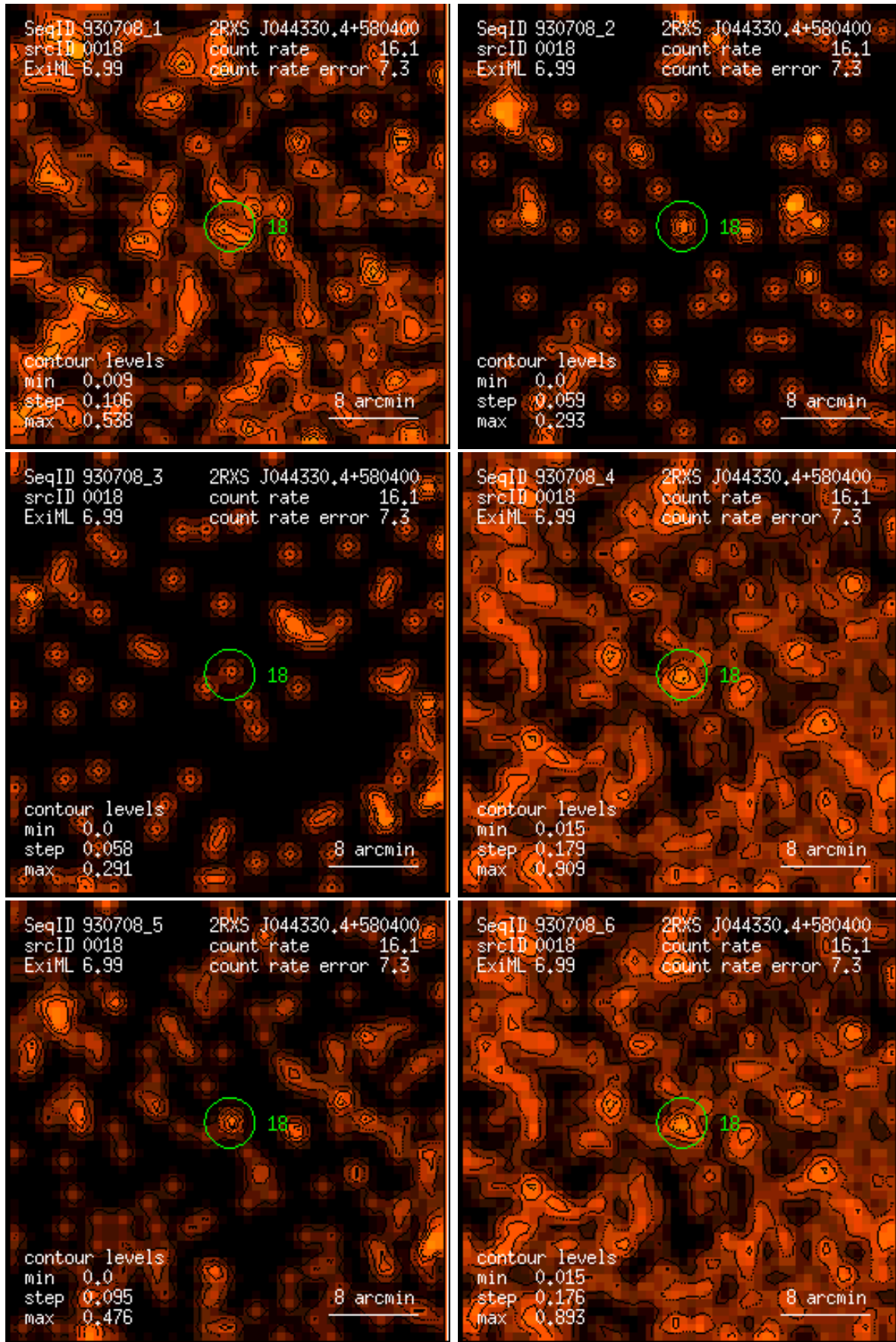
Figure 18: RASS 930708: detection 0018: band rate images, Gaussian filter: (1) PSPC channels 11 – 41, (2) 52 – 90, (3) 91 – 201, (4) 11 – 235, (5) 52 – 201, (6) 11 – 201. Broad band rates in counts/ks. Band rate contour levels in counts/ks/arcmin 2 .
