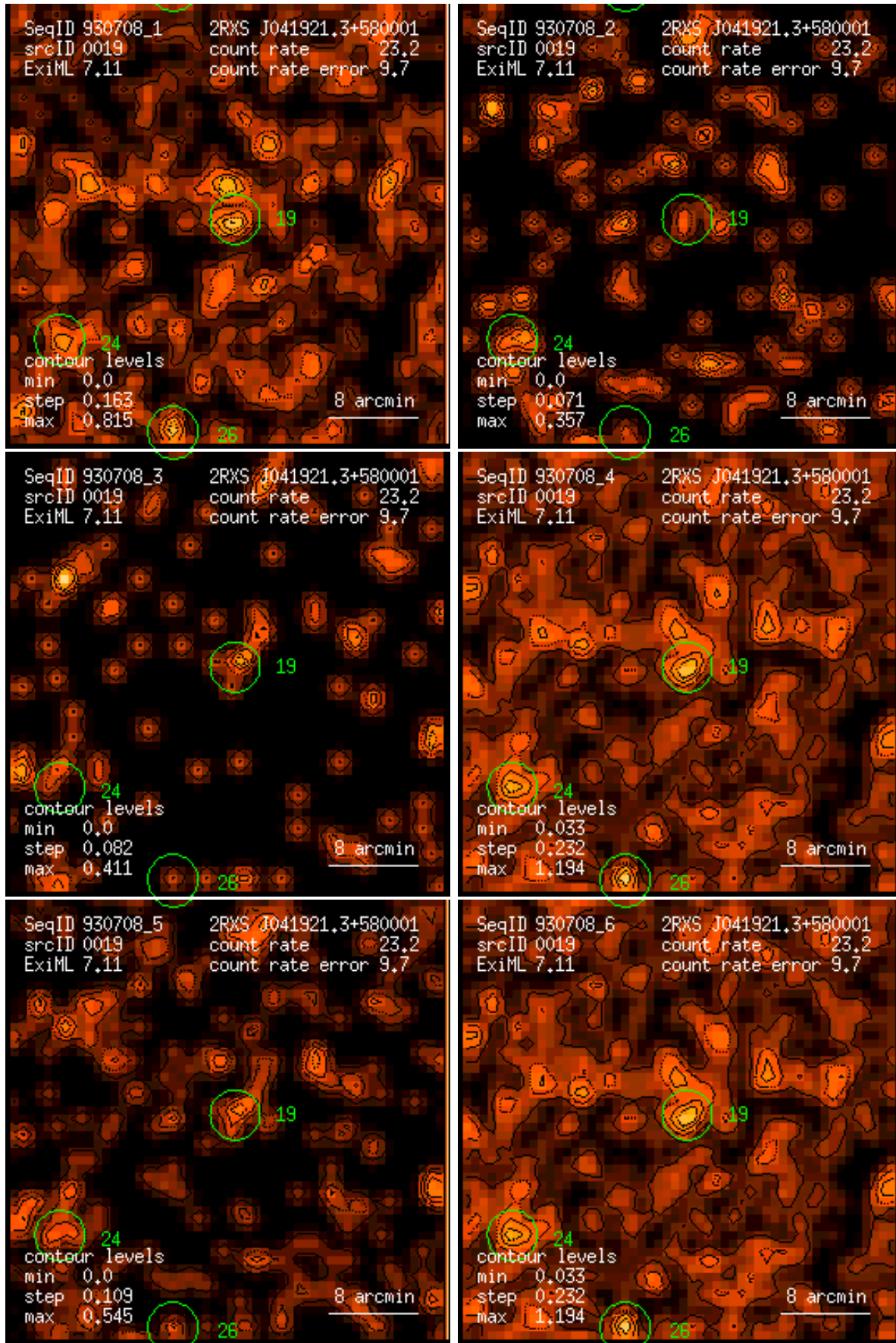
Figure 19: RASS 930708: detection 0019: band rate images, Gaussian filter: (1) PSPC channels 11 – 41, (2) 52 – 90, (3) 91 – 201, (4) 11 – 235, (5) 52 – 201, (6) 11 – 201. Broad band rates in counts/ks. Band rate contour levels in counts/ks/arcmin 2 .
