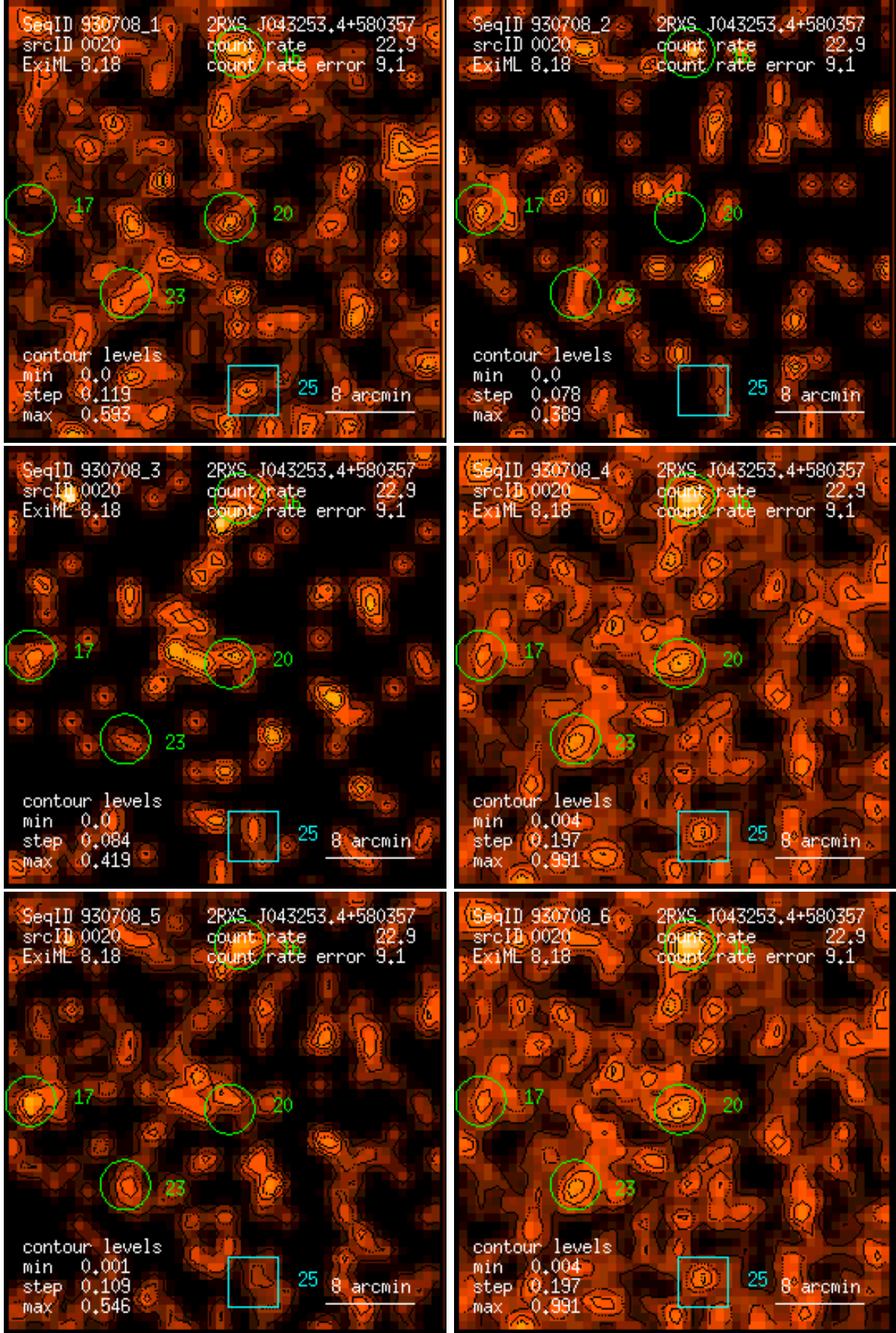
Figure 20: RASS 930708: detection 0020: band rate images, Gaussian filter: (1) PSPC channels 11 – 41, (2) 52 – 90, (3) 91 – 201, (4) 11 – 235, (5) 52 – 201, (6) 11 – 201. Broad band rates in counts/ks. Band rate contour levels in counts/ks/arcmin 2 .
