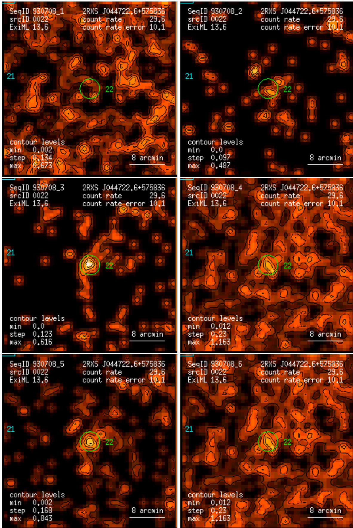
Figure 22: RASS 930708: detection 0022: band rate images, Gaussian filter: (1) PSPC channels 11 – 41, (2) 52 – 90, (3) 91 – 201, (4) 11 – 235, (5) 52 – 201, (6) 11 – 201. Broad band rates in counts/ks. Band rate contour levels in counts/ks/arcmin 2 .
