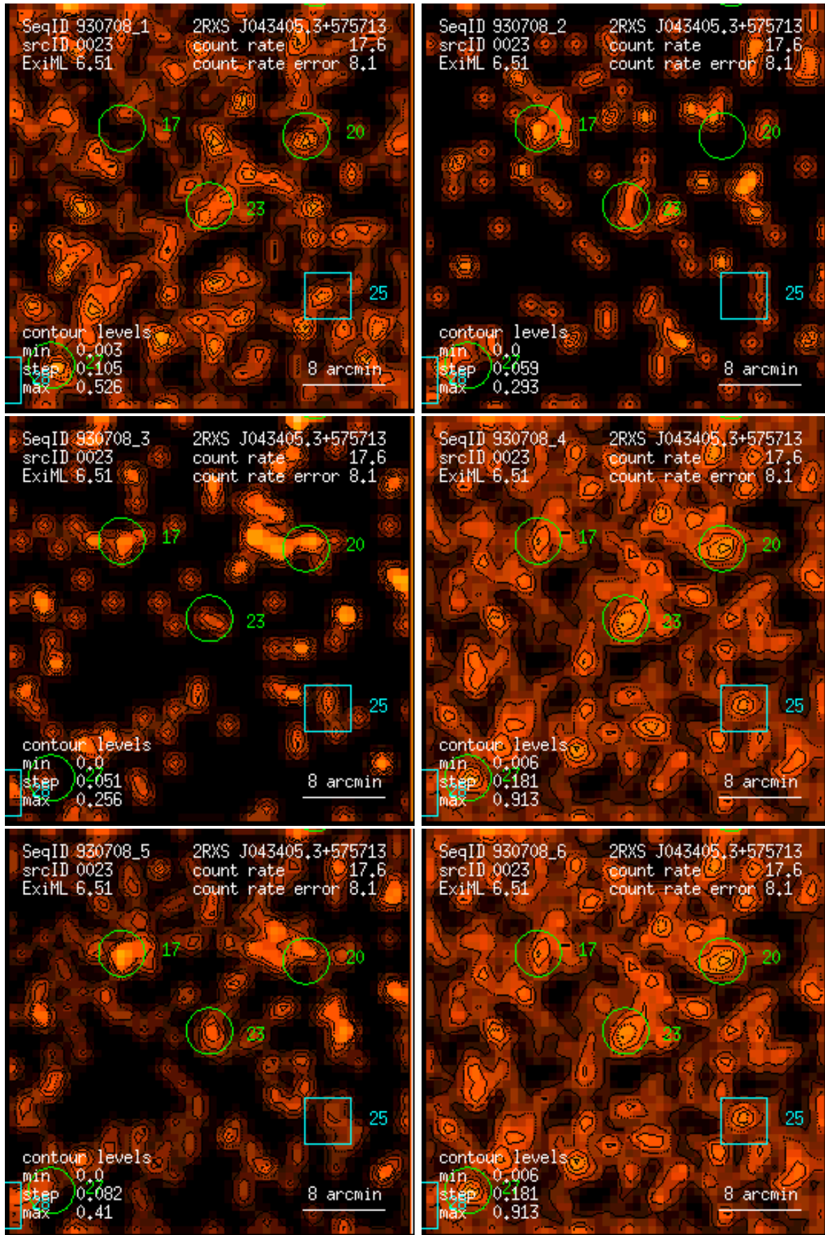
Figure 23: RASS 930708: detection 0023: band rate images, Gaussian filter: (1) PSPC channels 11 – 41, (2) 52 – 90, (3) 91 – 201, (4) 11 – 235, (5) 52 – 201, (6) 11 – 201. Broad band rates in counts/ks. Band rate contour levels in counts/ks/arcmin 2 .
