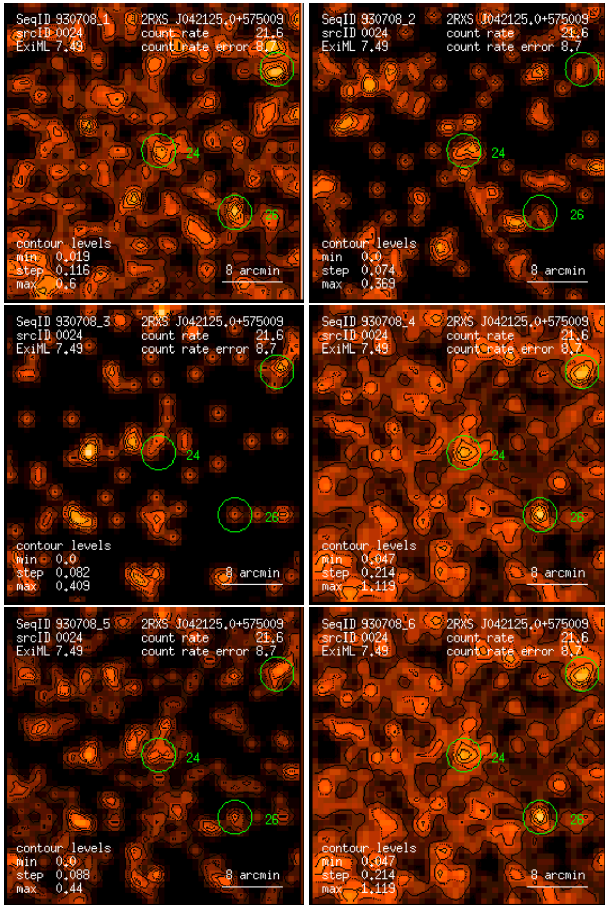
Figure 24: RASS 930708: detection 0024: band rate images, Gaussian filter: (1) PSPC channels 11 – 41, (2) 52 – 90, (3) 91 – 201, (4) 11 – 235, (5) 52 – 201, (6) 11 – 201. Broad band rates in counts/ks. Band rate contour levels in counts/ks/arcmin 2 .
