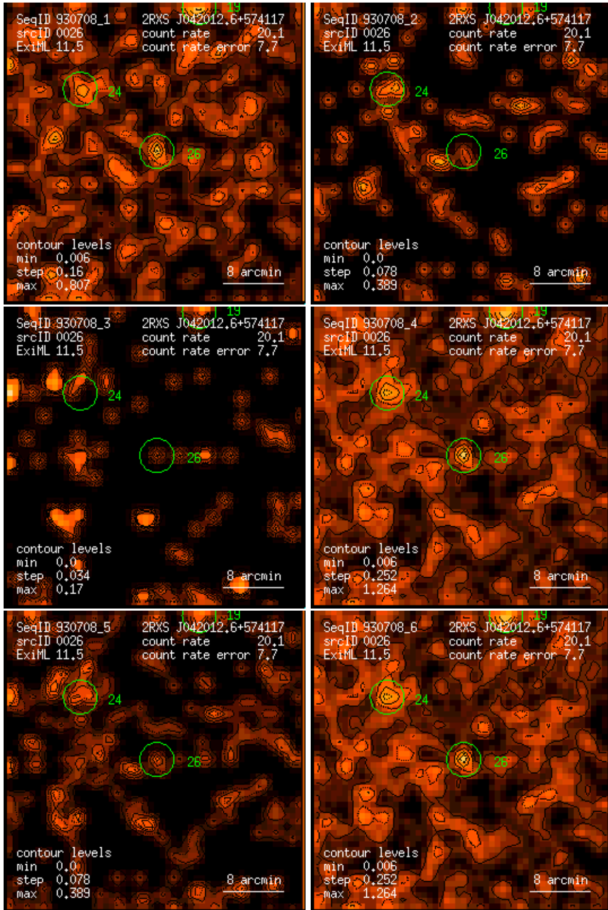
Figure 26: RASS 930708: detection 0026: band rate images, Gaussian filter: (1) PSPC channels 11 – 41, (2) 52 – 90, (3) 91 – 201, (4) 11 – 235, (5) 52 – 201, (6) 11 – 201. Broad band rates in counts/ks. Band rate contour levels in counts/ks/arcmin 2 .
