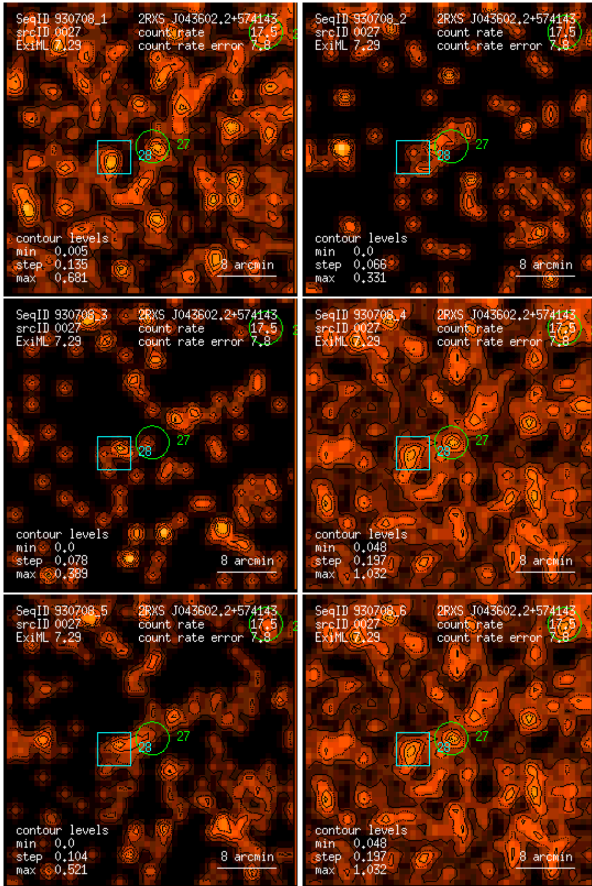
Figure 27: RASS 930708: detection 0027: band rate images, Gaussian filter: (1) PSPC channels 11 – 41, (2) 52 – 90, (3) 91 – 201, (4) 11 – 235, (5) 52 – 201, (6) 11 – 201. Broad band rates in counts/ks. Band rate contour levels in counts/ks/arcmin 2 .
