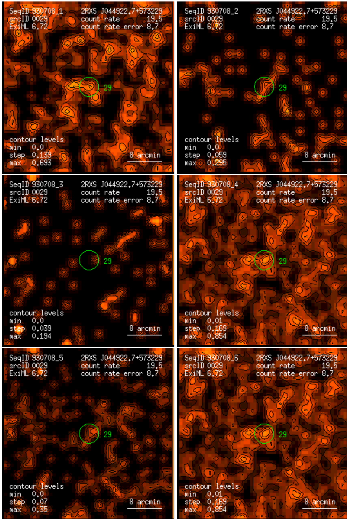
Figure 29: RASS 930708: detection 0029: band rate images, Gaussian filter: (1) PSPC channels 11 – 41, (2) 52 – 90, (3) 91 – 201, (4) 11 – 235, (5) 52 – 201, (6) 11 – 201. Broad band rates in counts/ks. Band rate contour levels in counts/ks/arcmin 2 .
