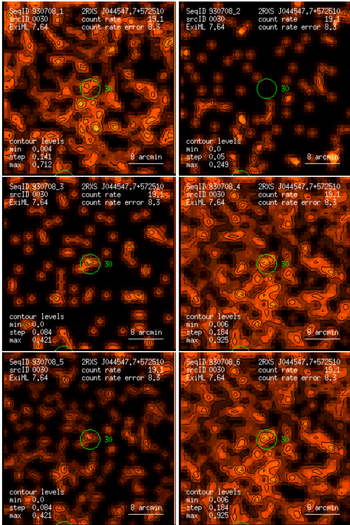
Figure 30: RASS 930708: detection 0030: band rate images, Gaussian filter: (1) PSPC channels 11 – 41, (2) 52 – 90, (3) 91 – 201, (4) 11 – 235, (5) 52 – 201, (6) 11 – 201. Broad band rates in counts/ks. Band rate contour levels in counts/ks/arcmin 2 .
