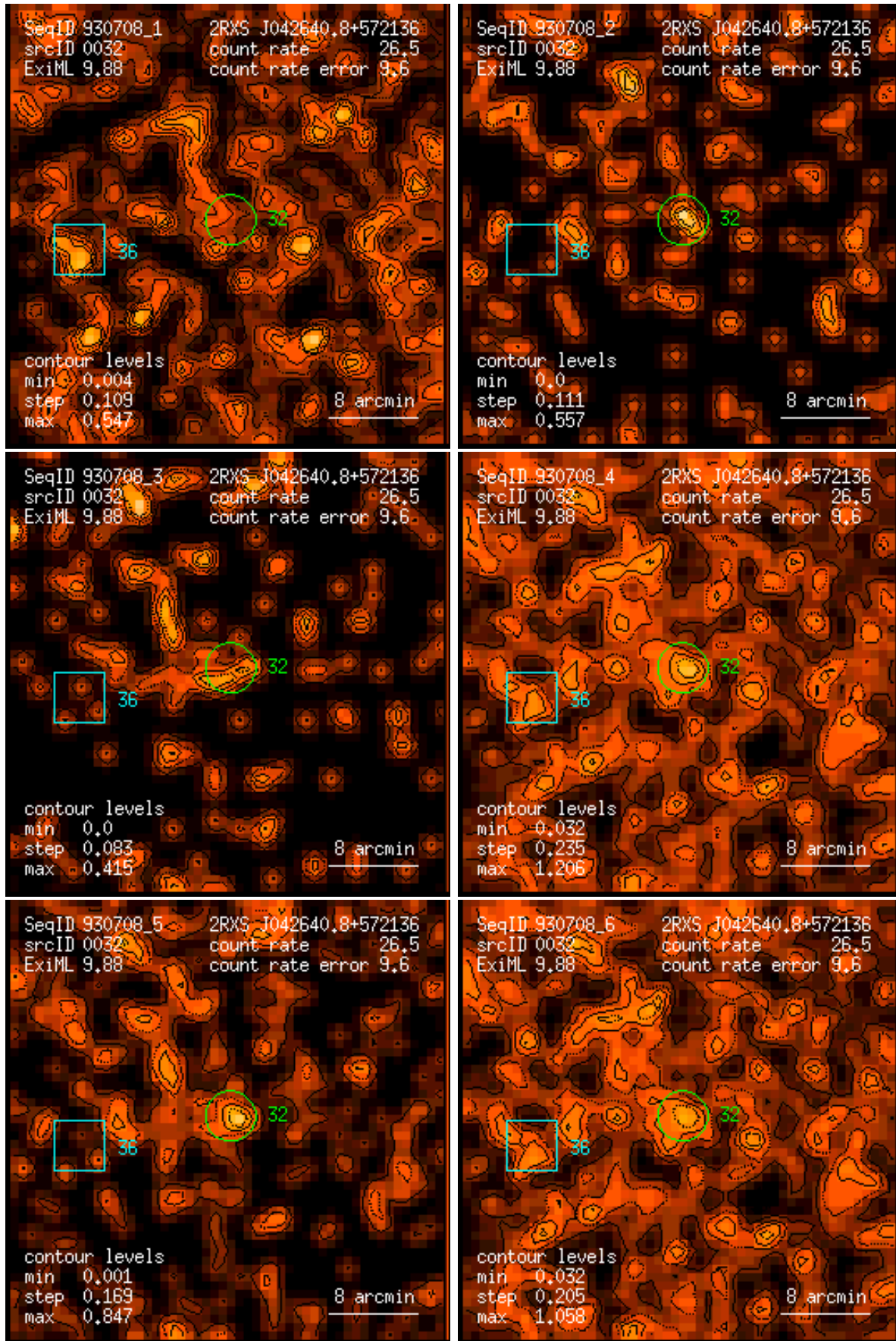
Figure 32: RASS 930708: detection 0032: band rate images, Gaussian filter: (1) PSPC channels 11 – 41, (2) 52 – 90, (3) 91 – 201, (4) 11 – 235, (5) 52 – 201, (6) 11 – 201. Broad band rates in counts/ks. Band rate contour levels in counts/ks/arcmin 2 .
