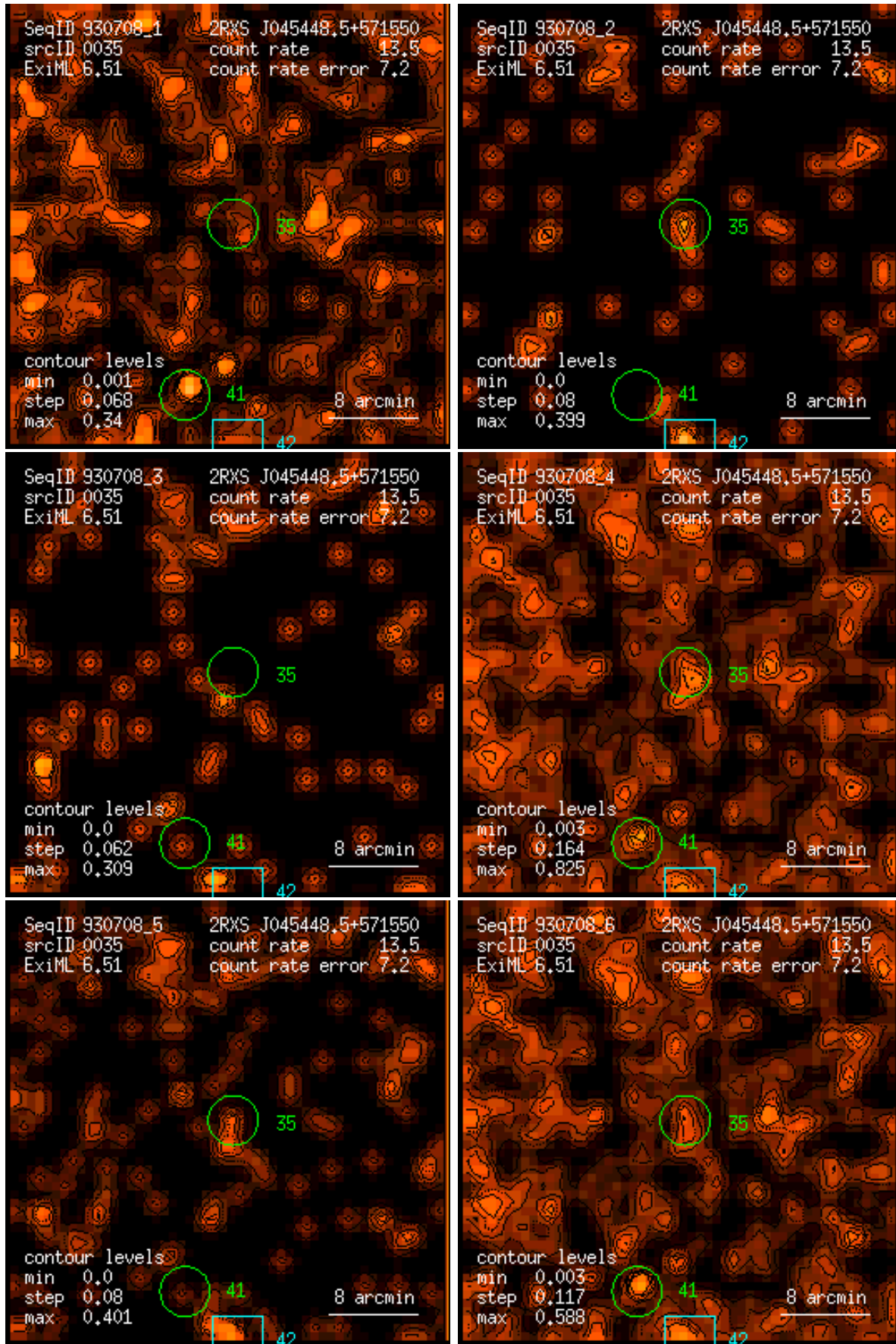
Figure 35: RASS 930708: detection 0035: band rate images, Gaussian filter: (1) PSPC channels 11 – 41, (2) 52 – 90, (3) 91 – 201, (4) 11 – 235, (5) 52 – 201, (6) 11 – 201. Broad band rates in counts/ks. Band rate contour levels in counts/ks/arcmin 2 .
