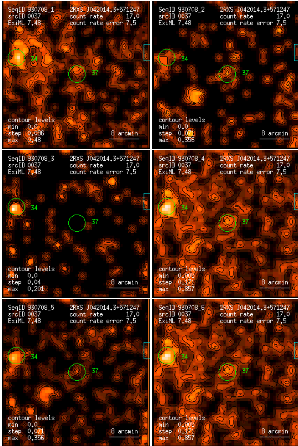
Figure 37: RASS 930708: detection 0037: band rate images, Gaussian filter: (1) PSPC channels 11 – 41, (2) 52 – 90, (3) 91 – 201, (4) 11 – 235, (5) 52 – 201, (6) 11 – 201. Broad band rates in counts/ks. Band rate contour levels in counts/ks/arcmin 2 .
