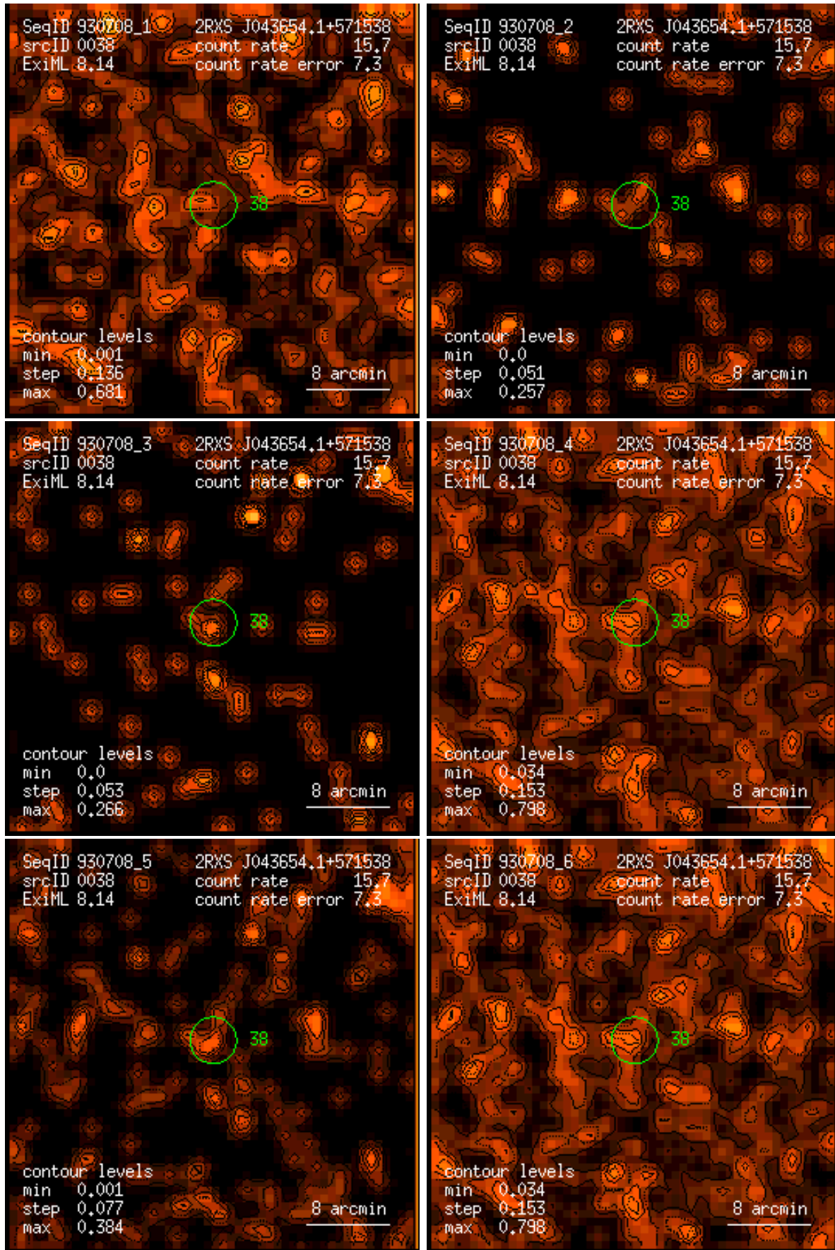
Figure 38: RASS 930708: detection 0038: band rate images, Gaussian filter: (1) PSPC channels 11 – 41, (2) 52 – 90, (3) 91 – 201, (4) 11 – 235, (5) 52 – 201, (6) 11 – 201. Broad band rates in counts/ks. Band rate contour levels in counts/ks/arcmin 2 .
