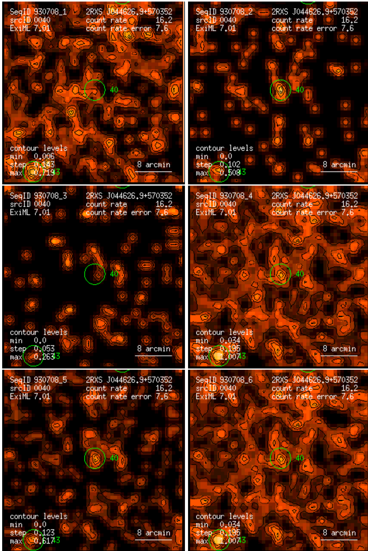
Figure 40: RASS 930708: detection 0040: band rate images, Gaussian filter: (1) PSPC channels 11 – 41, (2) 52 – 90, (3) 91 – 201, (4) 11 – 235, (5) 52 – 201, (6) 11 – 201. Broad band rates in counts/ks. Band rate contour levels in counts/ks/arcmin 2 .
