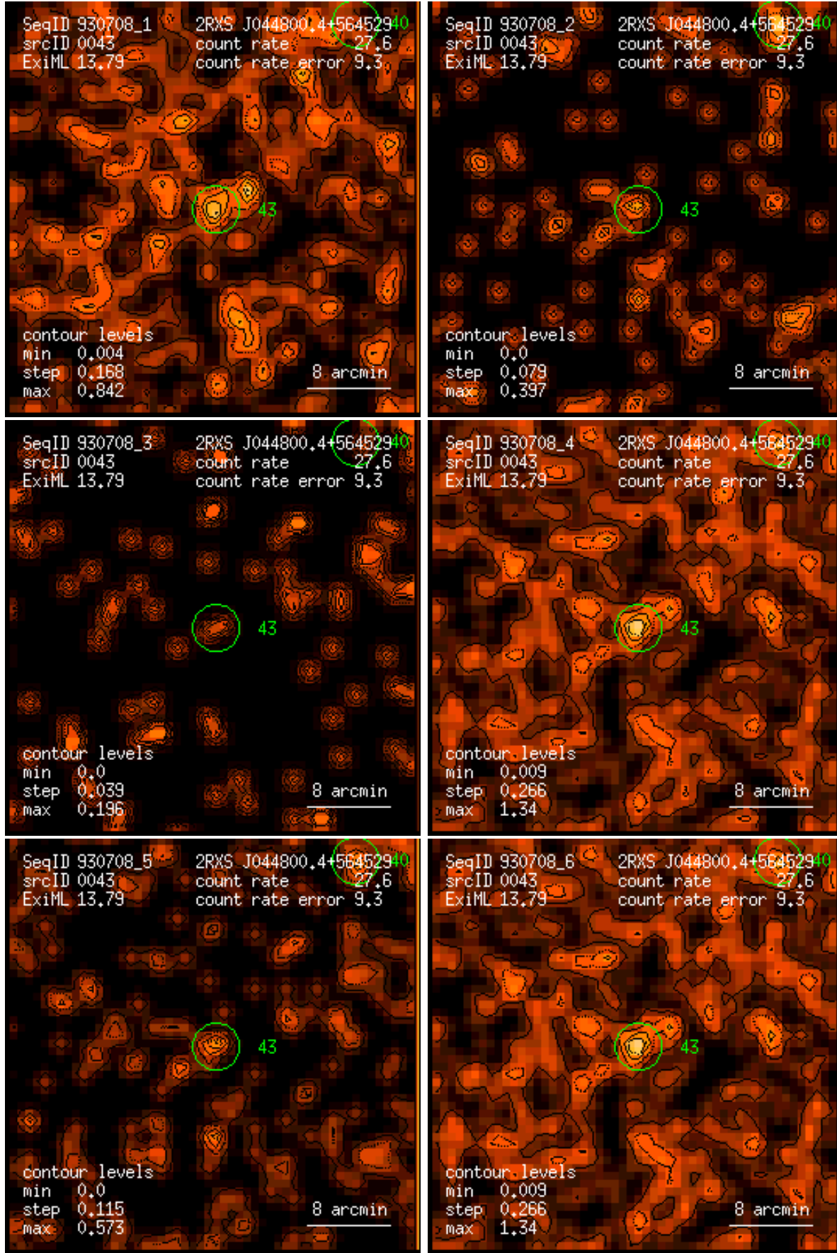
Figure 43: RASS 930708: detection 0043: band rate images, Gaussian filter: (1) PSPC channels 11 – 41, (2) 52 – 90, (3) 91 – 201, (4) 11 – 235, (5) 52 – 201, (6) 11 – 201. Broad band rates in counts/ks. Band rate contour levels in counts/ks/arcmin 2 .
