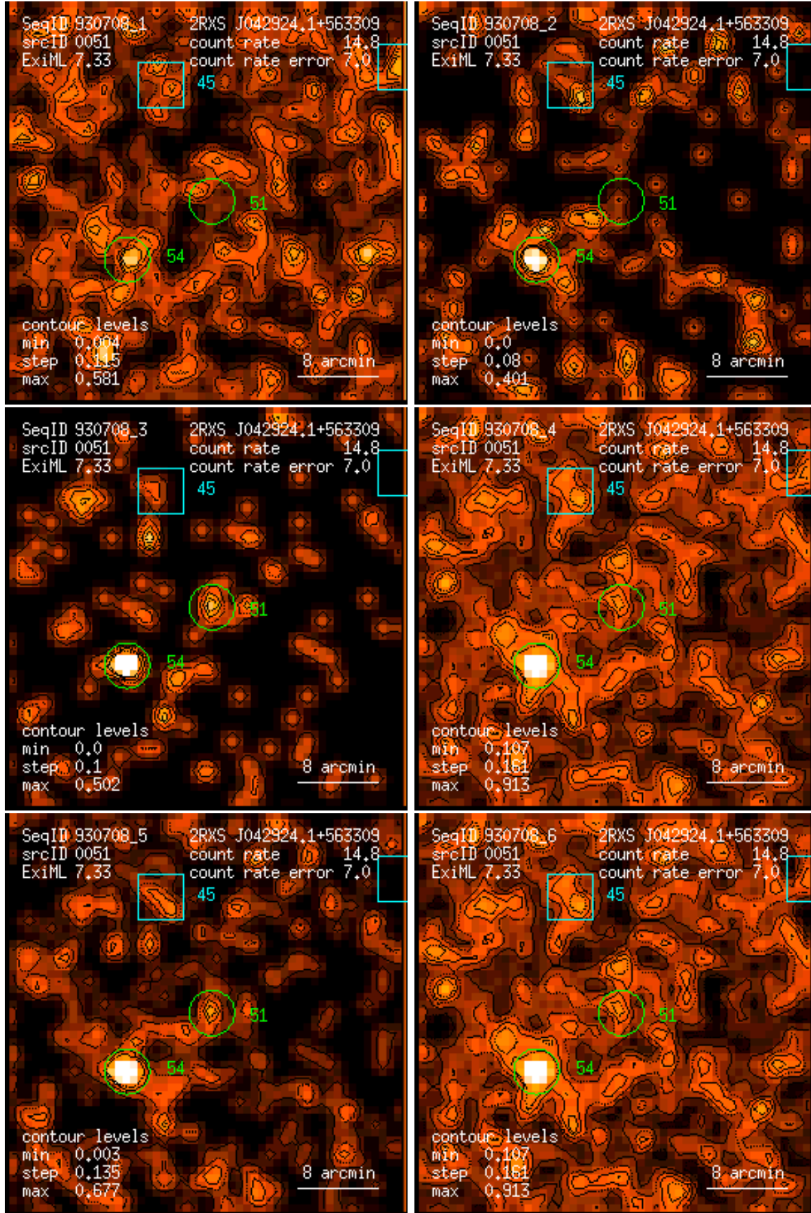
Figure 51: RASS 930708: detection 0051: band rate images, Gaussian filter: (1) PSPC channels 11 – 41, (2) 52 – 90, (3) 91 – 201, (4) 11 – 235, (5) 52 – 201, (6) 11 – 201. Broad band rates in counts/ks. Band rate contour levels in counts/ks/arcmin 2 .
