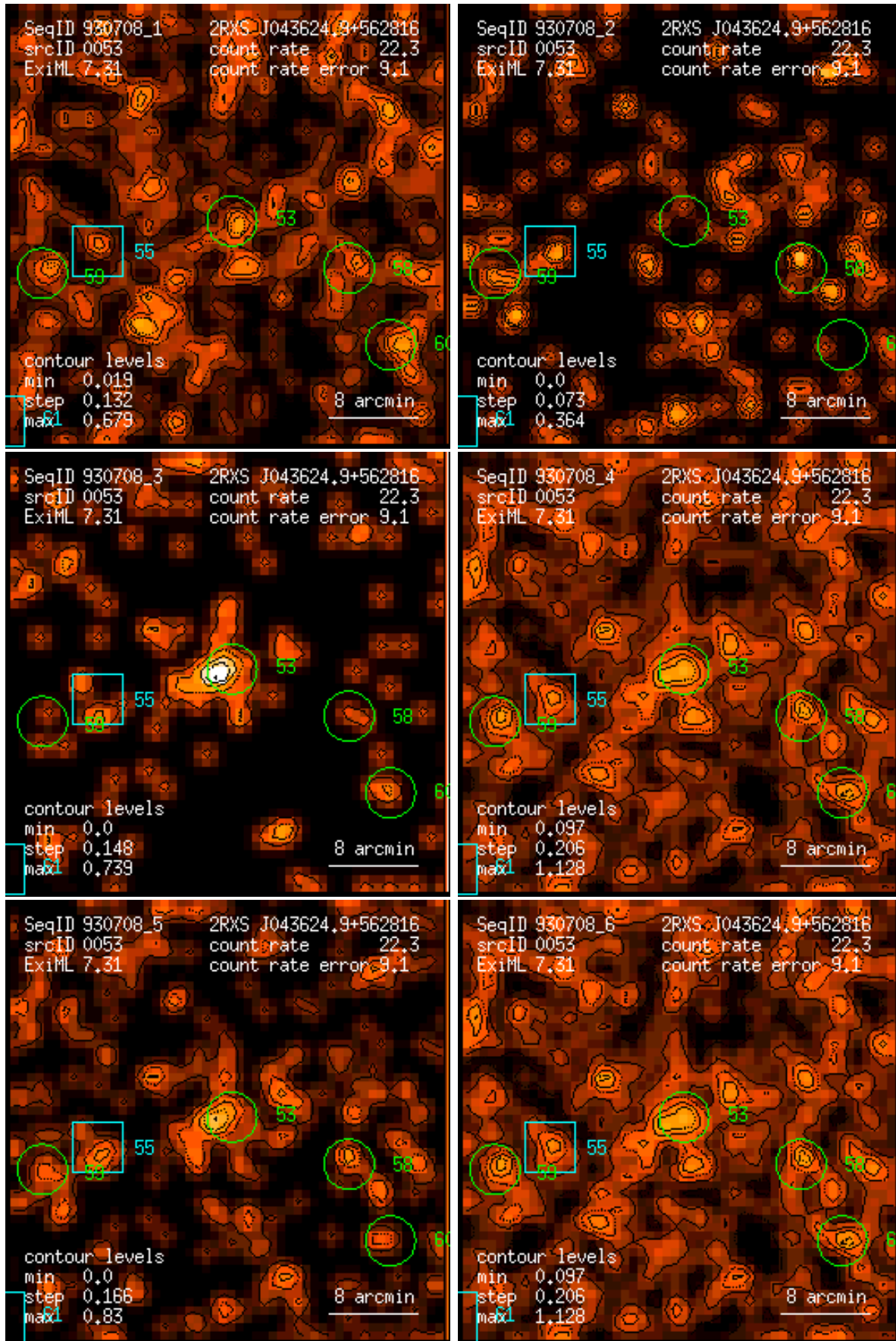
Figure 53: RASS 930708: detection 0053: band rate images, Gaussian filter: (1) PSPC channels 11 – 41, (2) 52 – 90, (3) 91 – 201, (4) 11 – 235, (5) 52 – 201, (6) 11 – 201. Broad band rates in counts/ks. Band rate contour levels in counts/ks/arcmin 2 .
