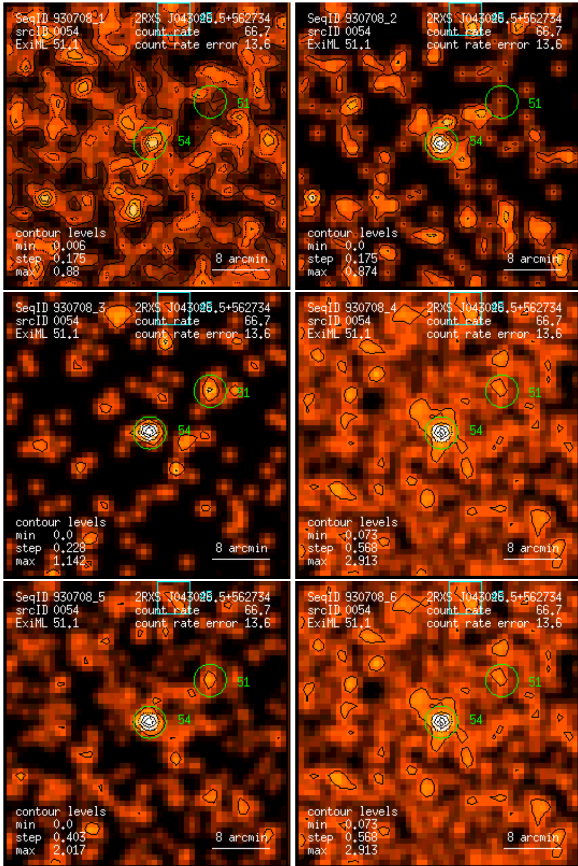
Figure 54: RASS 930708: detection 0054: band rate images, Gaussian filter: (1) PSPC channels 11 – 41, (2) 52 – 90, (3) 91 – 201, (4) 11 – 235, (5) 52 – 201, (6) 11 – 201. Broad band rates in counts/ks. Band rate contour levels in counts/ks/arcmin 2 .
