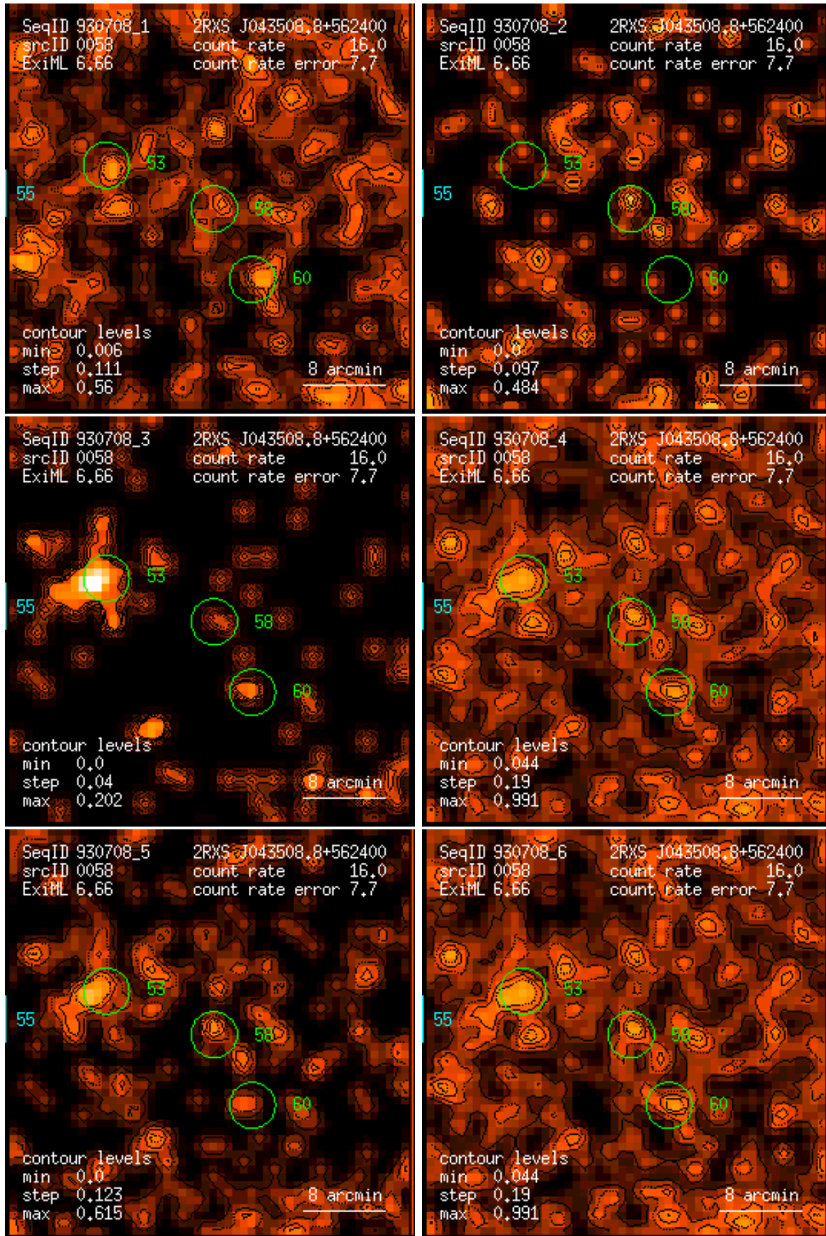
Figure 58: RASS 930708: detection 0058: band rate images, Gaussian filter: (1) PSPC channels 11 – 41, (2) 52 – 90, (3) 91 – 201, (4) 11 – 235, (5) 52 – 201, (6) 11 – 201. Broad band rates in counts/ks. Band rate contour levels in counts/ks/arcmin 2 .
