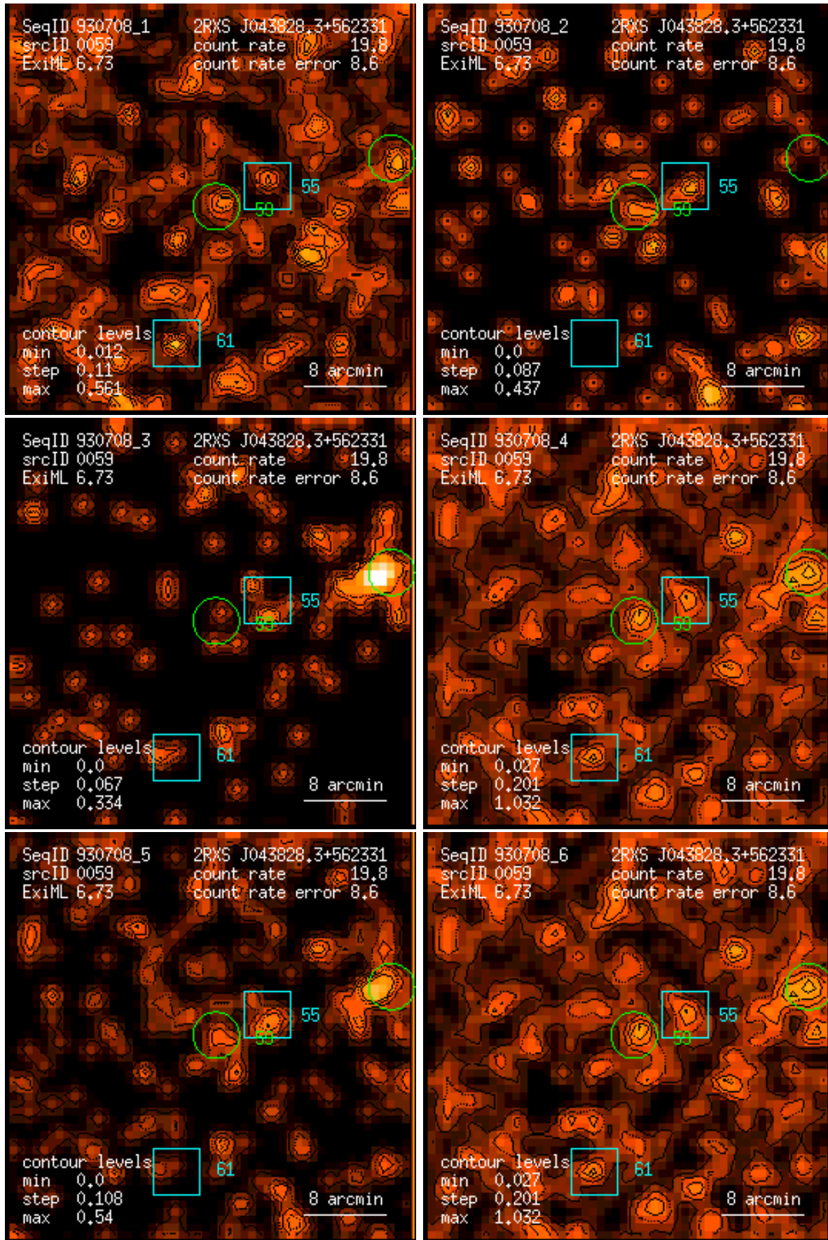
Figure 59: RASS 930708: detection 0059: band rate images, Gaussian filter: (1) PSPC channels 11 – 41, (2) 52 – 90, (3) 91 – 201, (4) 11 – 235, (5) 52 – 201, (6) 11 – 201. Broad band rates in counts/ks. Band rate contour levels in counts/ks/arcmin 2 .
