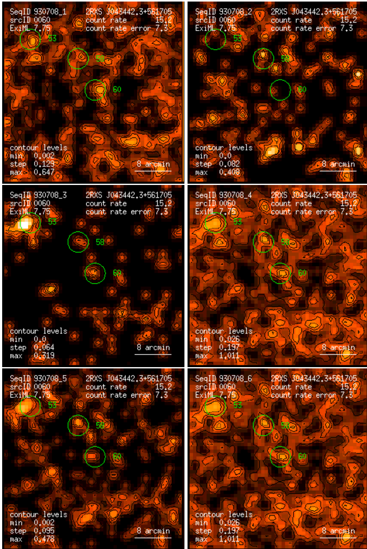
Figure 60: RASS 930708: detection 0060: band rate images, Gaussian filter: (1) PSPC channels 11 – 41, (2) 52 – 90, (3) 91 – 201, (4) 11 – 235, (5) 52 – 201, (6) 11 – 201. Broad band rates in counts/ks. Band rate contour levels in counts/ks/arcmin 2 .
