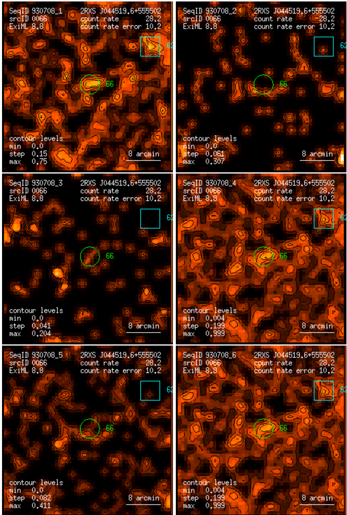
Figure 66: RASS 930708: detection 0066: band rate images, Gaussian filter: (1) PSPC channels 11 – 41, (2) 52 – 90, (3) 91 – 201, (4) 11 – 235, (5) 52 – 201, (6) 11 – 201. Broad band rates in counts/ks. Band rate contour levels in counts/ks/arcmin 2 .
