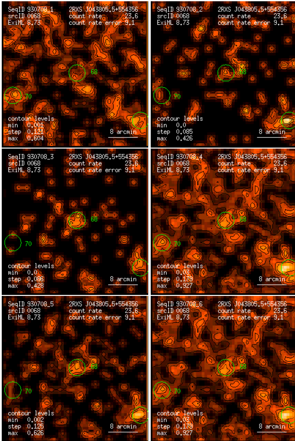
Figure 68: RASS 930708: detection 0068: band rate images, Gaussian filter: (1) PSPC channels 11 – 41, (2) 52 – 90, (3) 91 – 201, (4) 11 – 235, (5) 52 – 201, (6) 11 – 201. Broad band rates in counts/ks. Band rate contour levels in counts/ks/arcmin 2 .
