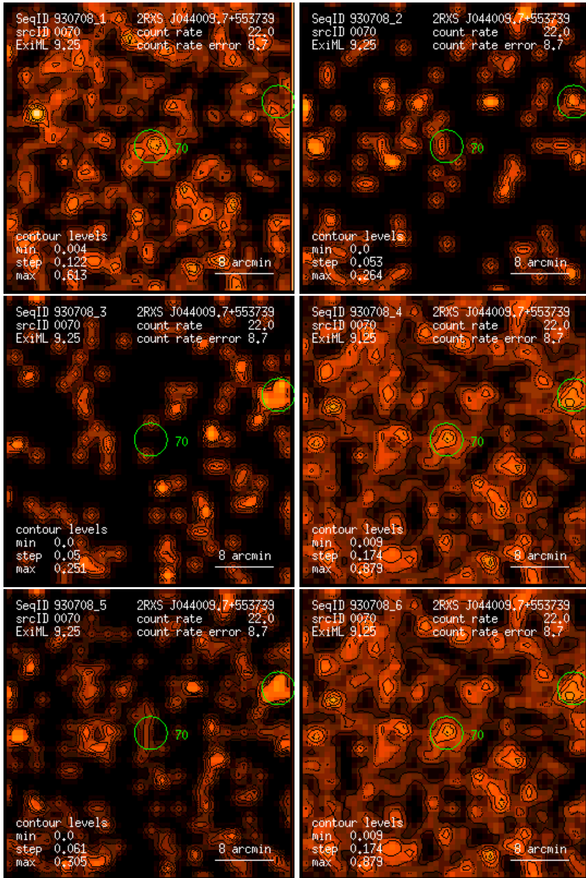
Figure 70: RASS 930708: detection 0070: band rate images, Gaussian filter: (1) PSPC channels 11 – 41, (2) 52 – 90, (3) 91 – 201, (4) 11 – 235, (5) 52 – 201, (6) 11 – 201. Broad band rates in counts/ks. Band rate contour levels in counts/ks/arcmin 2 .
