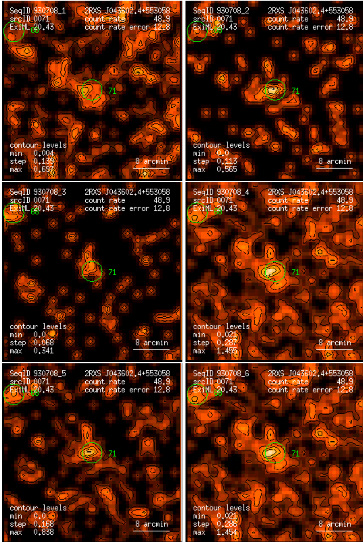
Figure 71: RASS 930708: detection 0071: band rate images, Gaussian filter: (1) PSPC channels 11 – 41, (2) 52 – 90, (3) 91 – 201, (4) 11 – 235, (5) 52 – 201, (6) 11 – 201. Broad band rates in counts/ks. Band rate contour levels in counts/ks/arcmin 2 .
