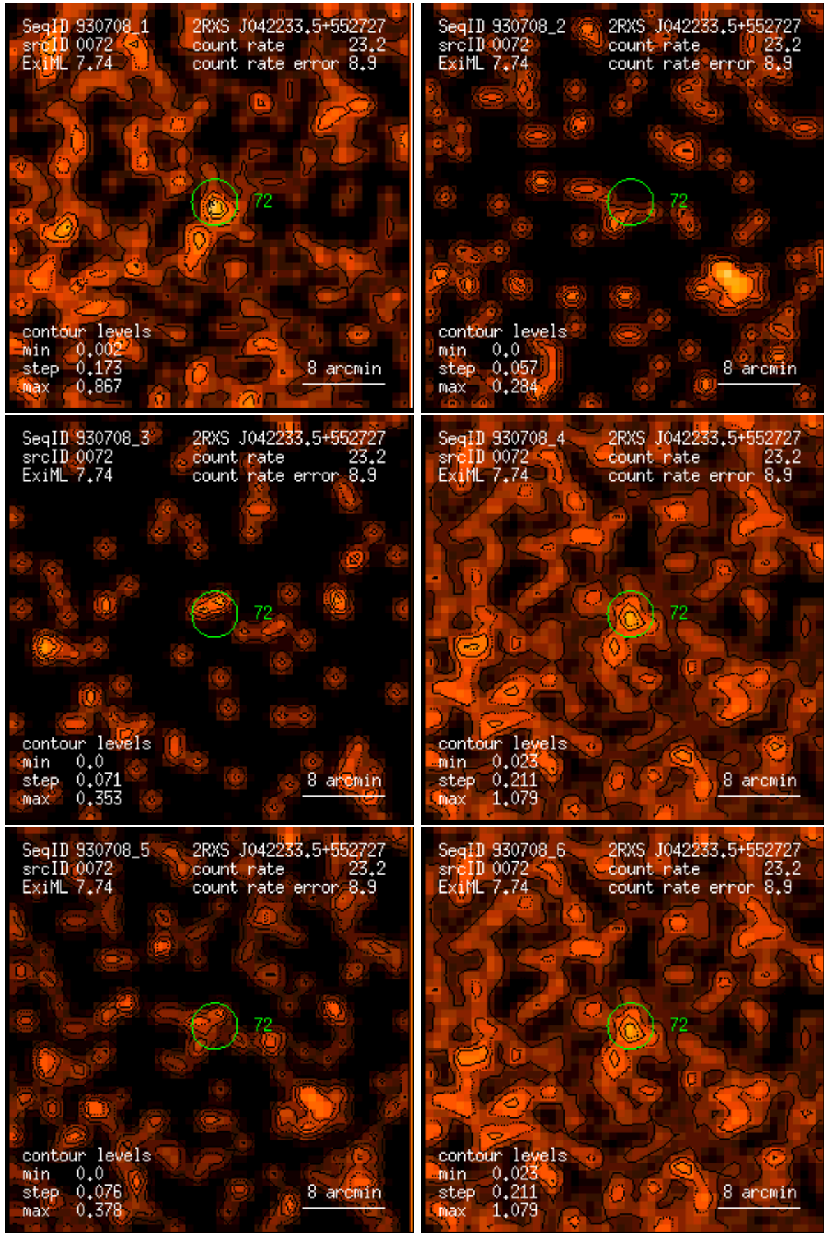
Figure 72: RASS 930708: detection 0072: band rate images, Gaussian filter: (1) PSPC channels 11 – 41, (2) 52 – 90, (3) 91 – 201, (4) 11 – 235, (5) 52 – 201, (6) 11 – 201. Broad band rates in counts/ks. Band rate contour levels in counts/ks/arcmin 2 .
