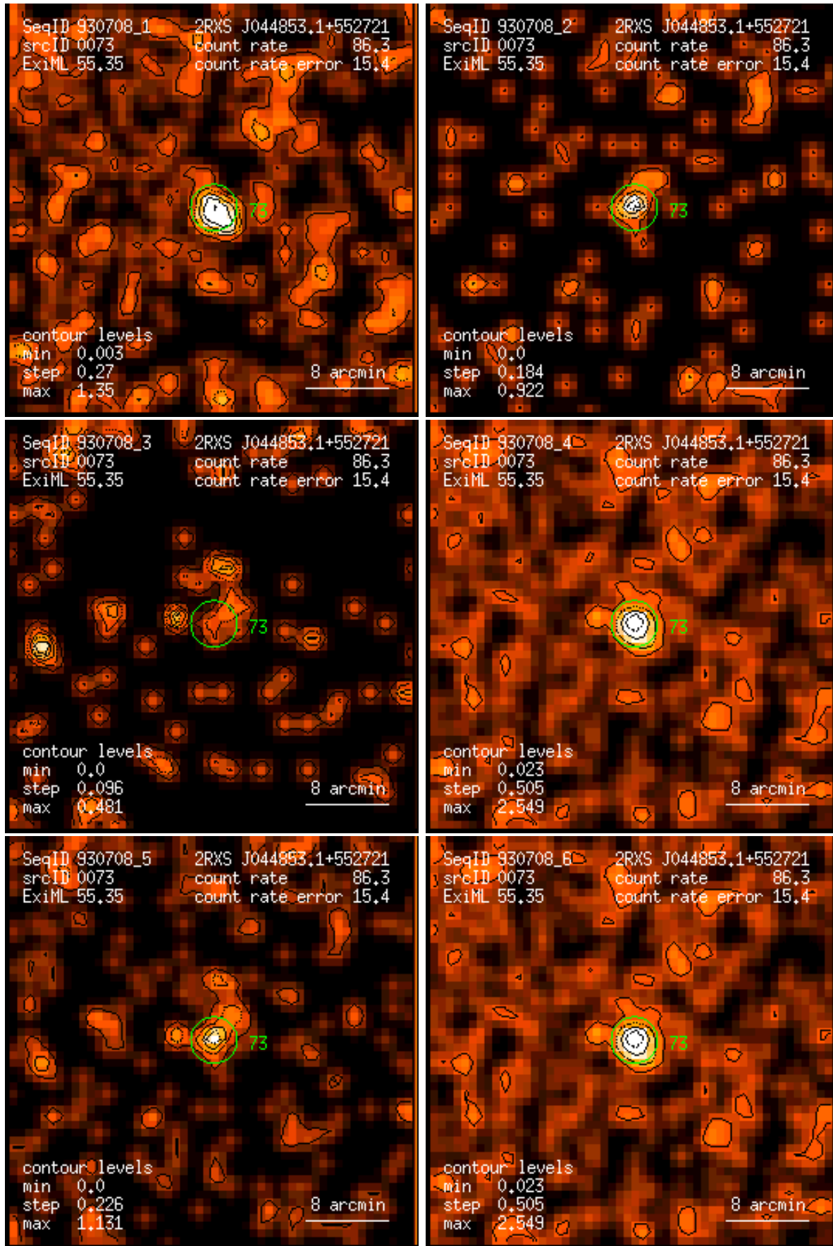
Figure 73: RASS 930708: detection 0073: band rate images, Gaussian filter: (1) PSPC channels 11 – 41, (2) 52 – 90, (3) 91 – 201, (4) 11 – 235, (5) 52 – 201, (6) 11 – 201. Broad band rates in counts/ks. Band rate contour levels in counts/ks/arcmin 2 .
