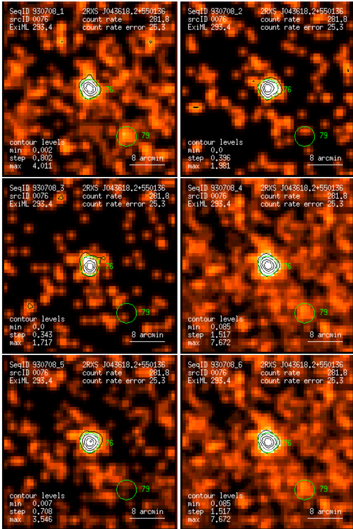
Figure 76: RASS 930708: detection 0076: band rate images, Gaussian filter: (1) PSPC channels 11 – 41, (2) 52 – 90, (3) 91 – 201, (4) 11 – 235, (5) 52 – 201, (6) 11 – 201. Broad band rates in counts/ks. Band rate contour levels in counts/ks/arcmin 2 .
