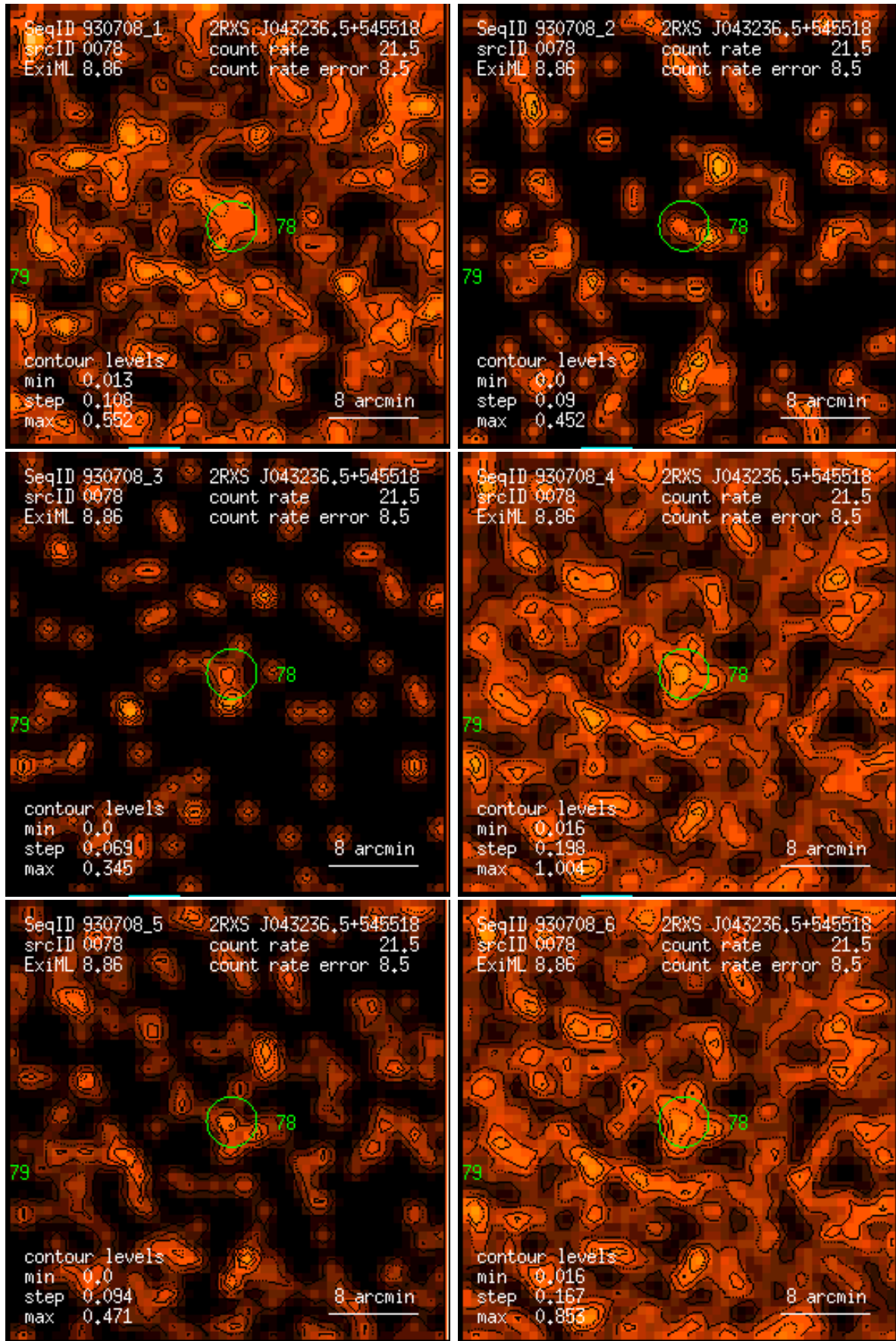
Figure 78: RASS 930708: detection 0078: band rate images, Gaussian filter: (1) PSPC channels 11 – 41, (2) 52 – 90, (3) 91 – 201, (4) 11 – 235, (5) 52 – 201, (6) 11 – 201. Broad band rates in counts/ks. Band rate contour levels in counts/ks/arcmin 2 .
