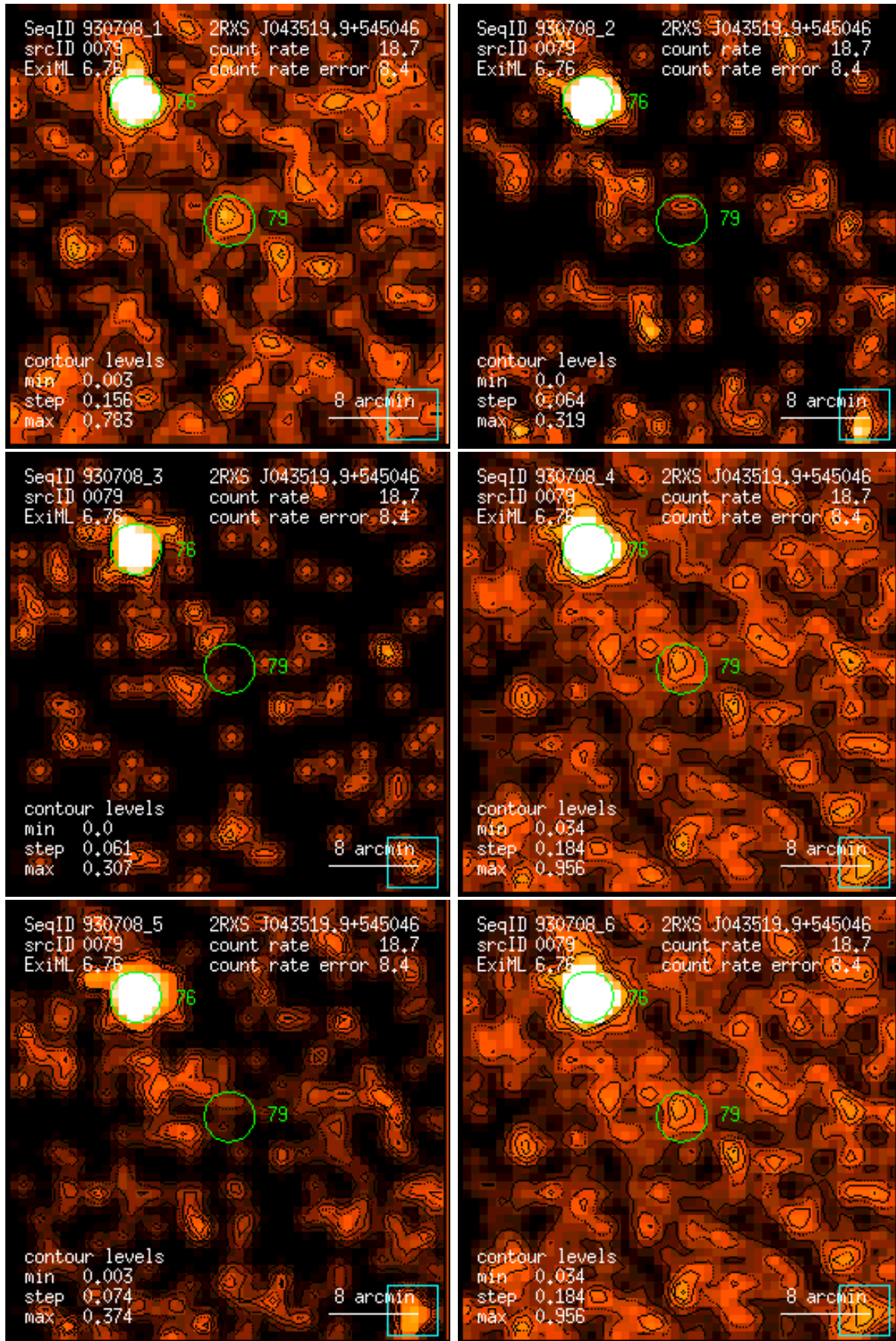
Figure 79: RASS 930708: detection 0079: band rate images, Gaussian filter: (1) PSPC channels 11 – 41, (2) 52 – 90, (3) 91 – 201, (4) 11 – 235, (5) 52 – 201, (6) 11 – 201. Broad band rates in counts/ks. Band rate contour levels in counts/ks/arcmin 2 .
