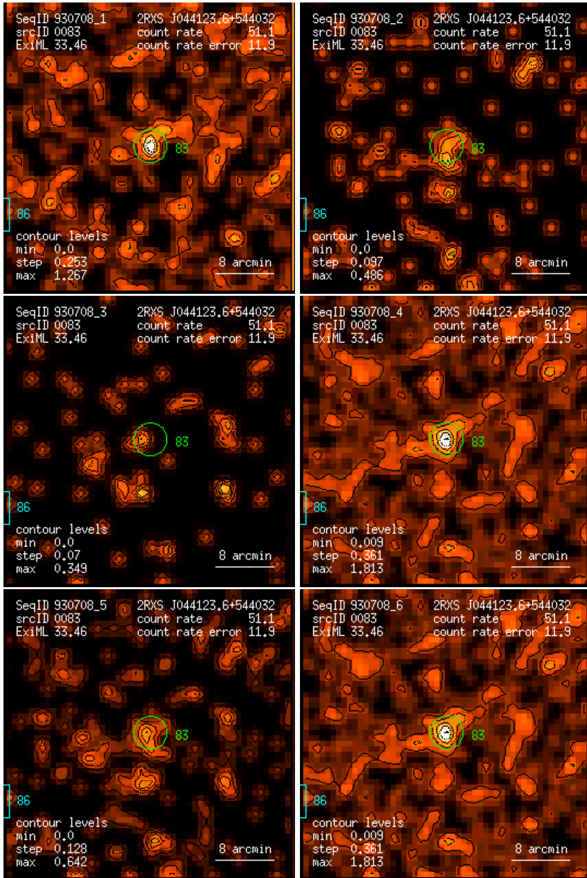
Figure 83: RASS 930708: detection 0083: band rate images, Gaussian filter: (1) PSPC channels 11 – 41, (2) 52 – 90, (3) 91 – 201, (4) 11 – 235, (5) 52 – 201, (6) 11 – 201. Broad band rates in counts/ks. Band rate contour levels in counts/ks/arcmin 2 .
