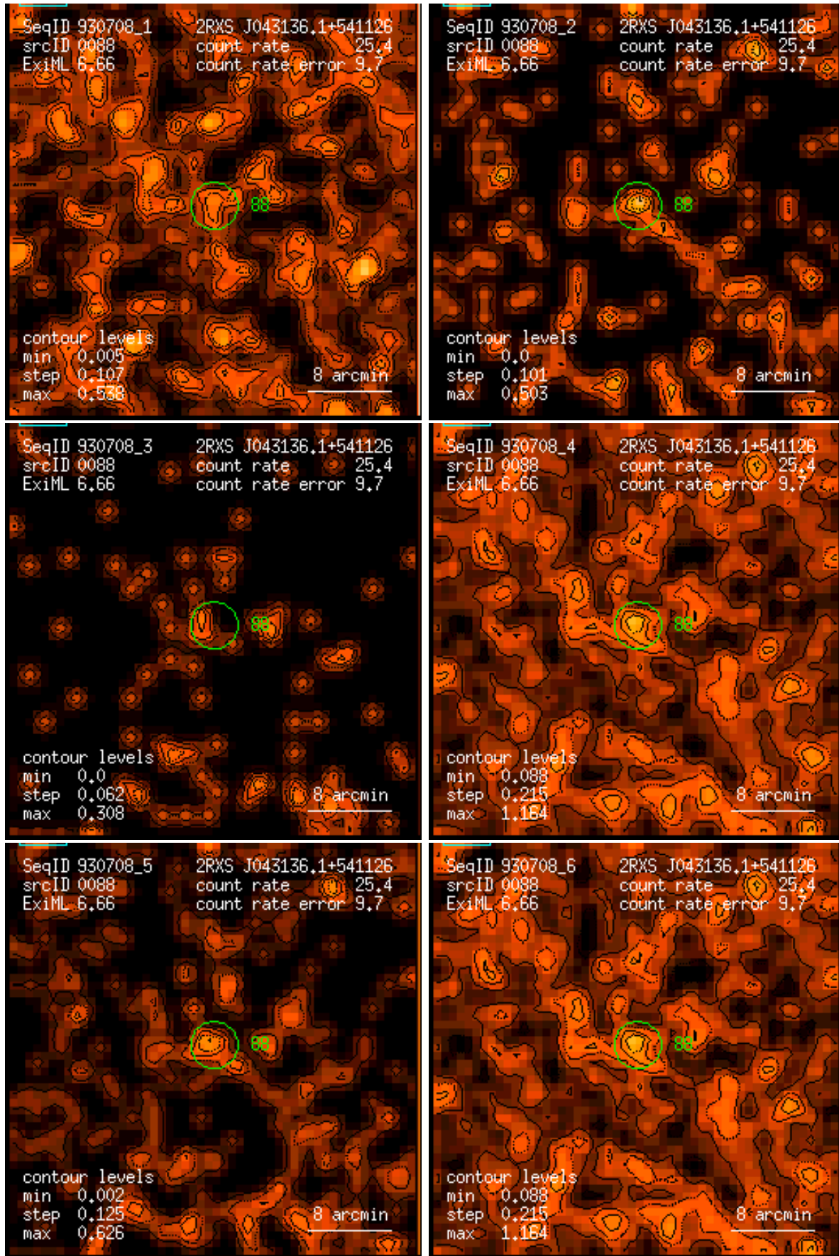
Figure 88: RASS 930708: detection 0088: band rate images, Gaussian filter: (1) PSPC channels 11 – 41, (2) 52 – 90, (3) 91 – 201, (4) 11 – 235, (5) 52 – 201, (6) 11 – 201. Broad band rates in counts/ks. Band rate contour levels in counts/ks/arcmin 2 .
