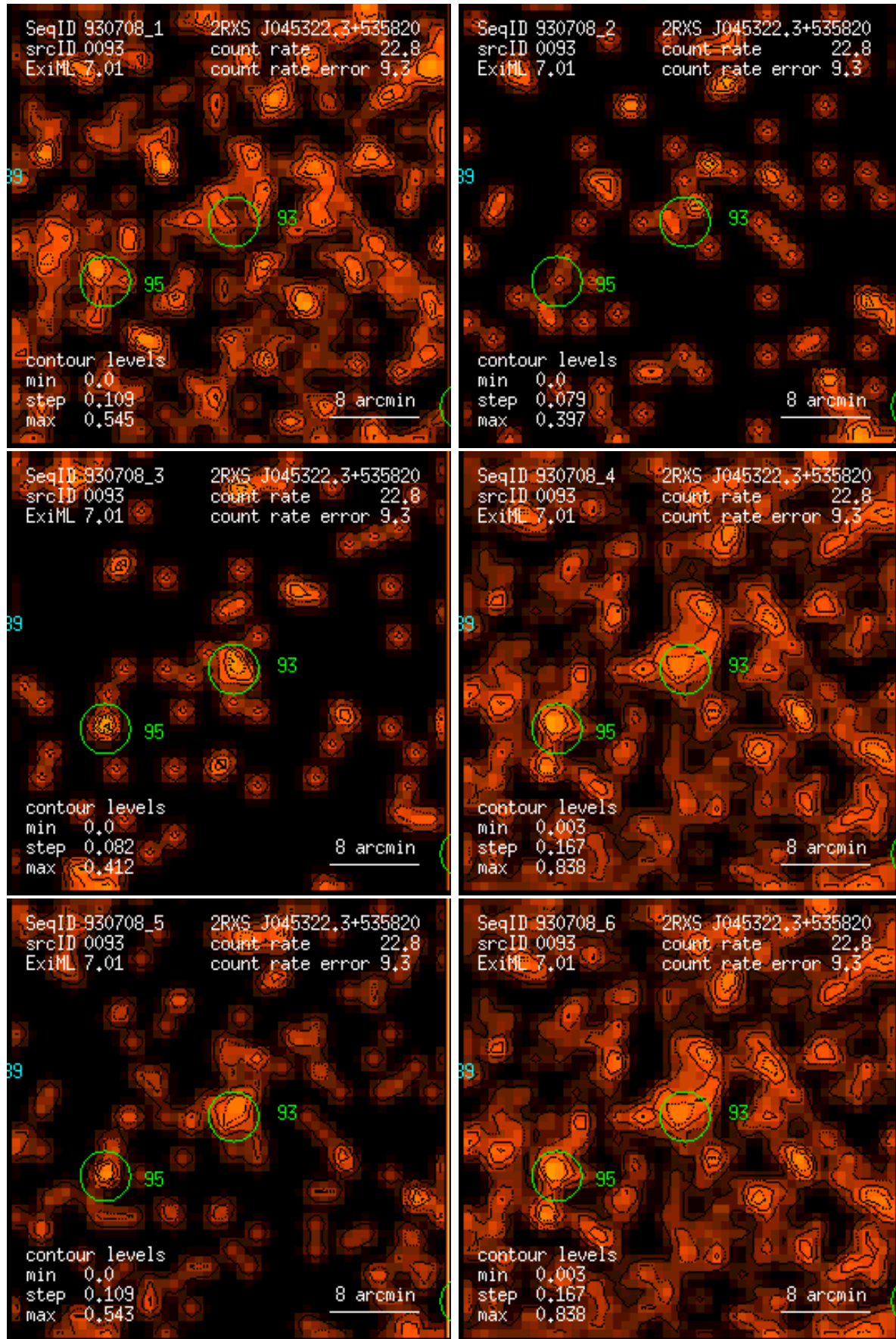
Figure 93: RASS 930708: detection 0093: band rate images, Gaussian filter: (1) PSPC channels 11 – 41, (2) 52 – 90, (3) 91 – 201, (4) 11 – 235, (5) 52 – 201, (6) 11 – 201. Broad band rates in counts/ks. Band rate contour levels in counts/ks/arcmin 2 .
