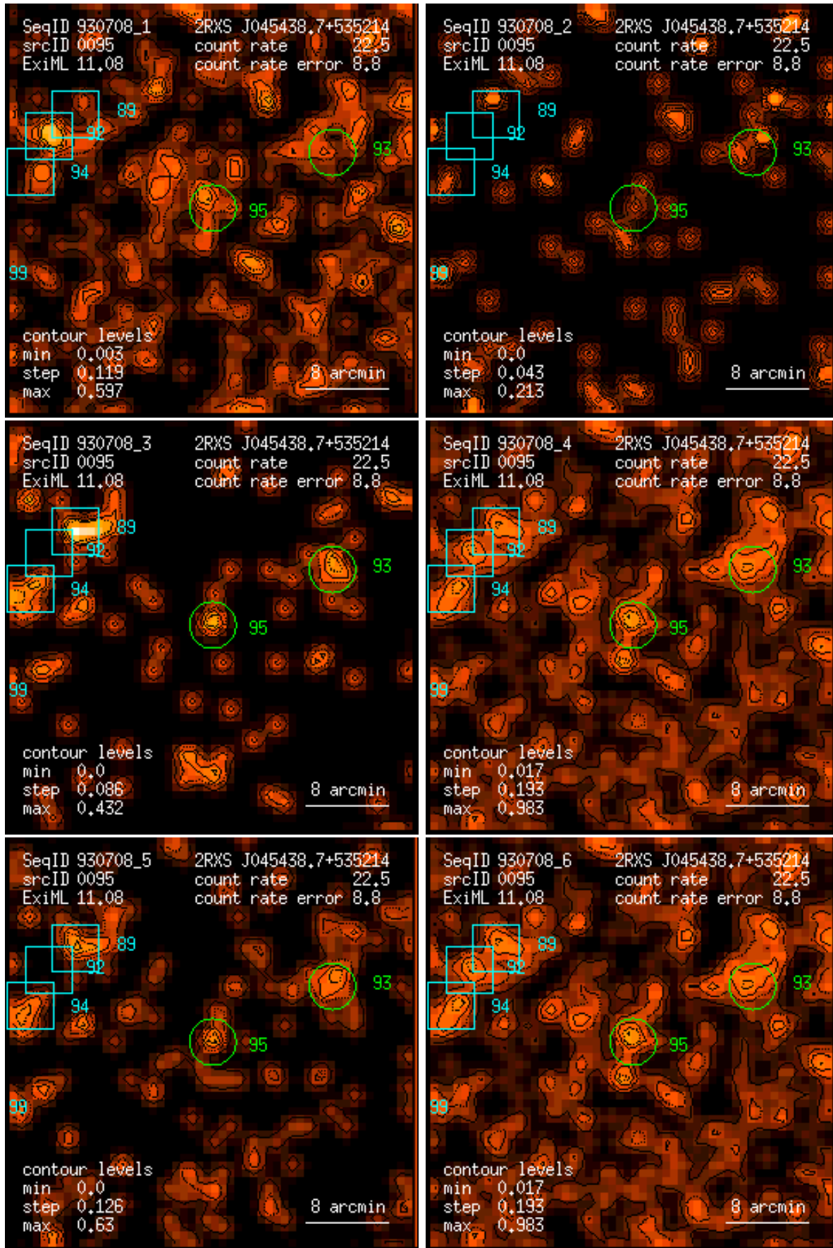
Figure 95: RASS 930708: detection 0095: band rate images, Gaussian filter: (1) PSPC channels 11 – 41, (2) 52 – 90, (3) 91 – 201, (4) 11 – 235, (5) 52 – 201, (6) 11 – 201. Broad band rates in counts/ks. Band rate contour levels in counts/ks/arcmin 2 .
