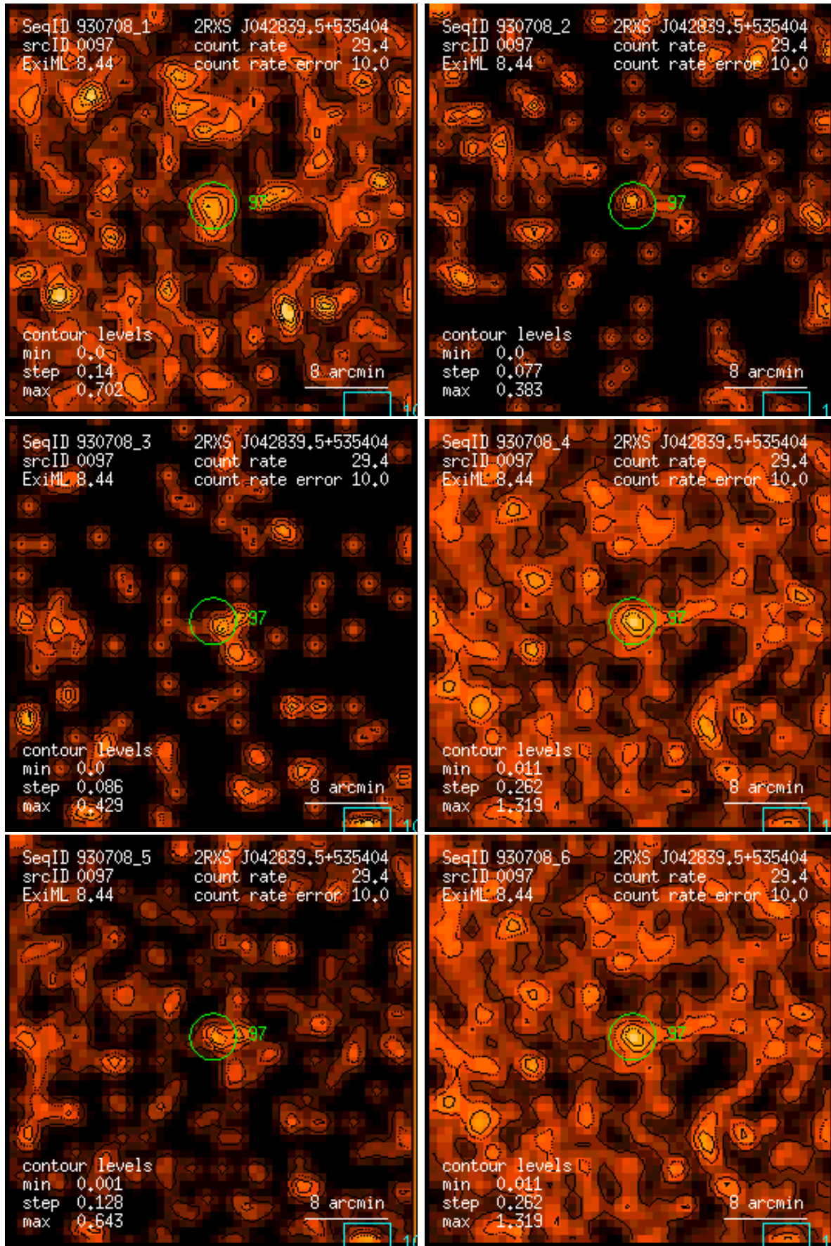
Figure 97: RASS 930708: detection 0097: band rate images, Gaussian filter: (1) PSPC channels 11 – 41, (2) 52 – 90, (3) 91 – 201, (4) 11 – 235, (5) 52 – 201, (6) 11 – 201. Broad band rates in counts/ks. Band rate contour levels in counts/ks/arcmin 2 .
